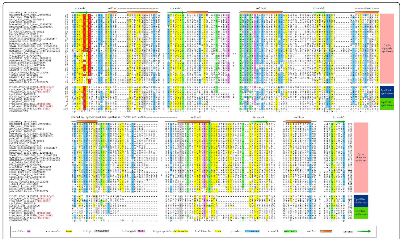
Figure 1 Alignment of the CDPs and class-I AatRS catalytic domains. Sequences are labeled by their gene names, species abbreviations and Genbank index numbers separated by underscores. PDB ids, if available, are also shown. Sequences are colored based on 85% consensus derived from an alignment of the cyclopeptide ligases. A key for the coloring scheme, consensus abbreviations and secondary structure labels is shown in the box below the alignment. Familial affiliations of the sequences are shown to the right. Species names are expanded in Abbreviations.
