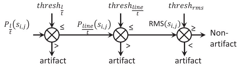
Figure 3 Schematics of the algorithm for the detection of low quality signals. The symbols (>) or (<) represent the cases where the feature was expected to be higher or lower than the specified threshold in order to determine if a given signal was labeled as artifact.
