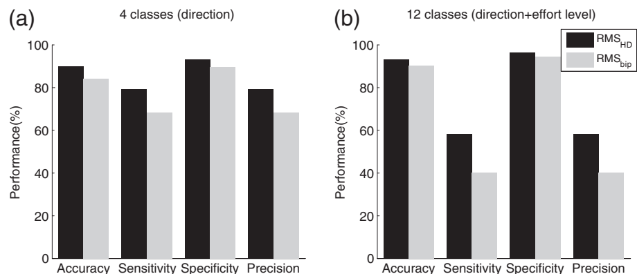
Figure 7 Classification performance using the feature RMS_{av-HD} (in black) extracted from HD-EMG maps or RMS_{av-bip} (in gray) extracted from single bipolar EMG signals. a) Four classes corresponding to type of task (flexion, extension, pronation and supination) or b) Twelve classes corresponding to type of task and effort level (10%, 30% or 50% MVC).
