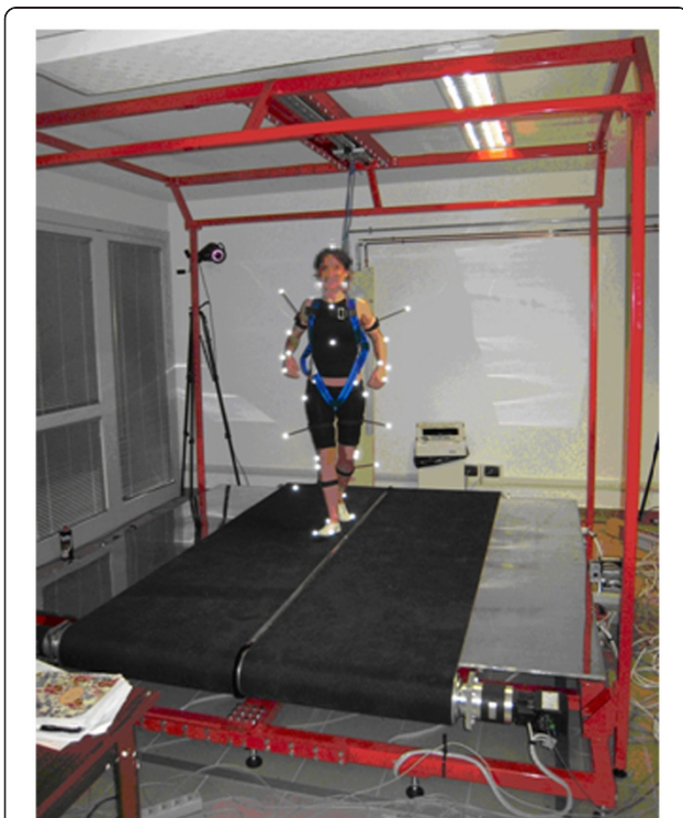
Figure 3 Picture of a subject while being on SENLY. SENLY with a tester attached to the tubular safety structure.
