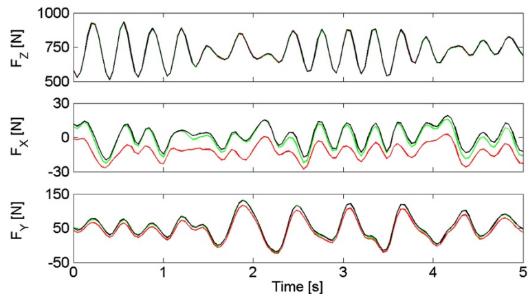
Figure 8 Recorded GRF after calibration. Representative 5-seconds-long record related of the set of forces developed by the operator while moving on the walkway during calibration procedures. The figure shows the components of GRF estimated by SENLY before (red) and after (green) calibrating, and compares them to those measured by the reference load cell (black). x, y and z axes are respectively the AP, ML and vertical directions.
