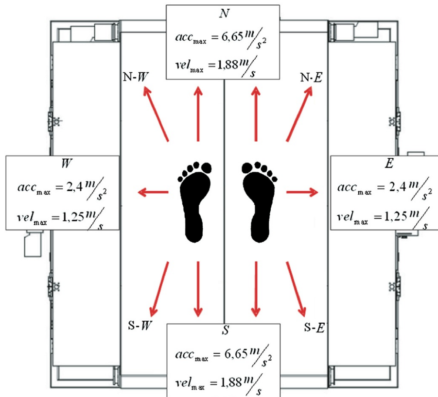
Figure 9 Perturbations. Kinematic features of the perturbations: North and South for both right and left feet; North-East, East and South-East for right foot; North-West, West and South-West for left foot. A perturbation consisted in: accelerating the belt up to the maximum speed, keeping the speed constant for a certain period, and stopping the belt. The N-W, N-E, S-W and S-E perturbations were obtained as a combination of the pure N, S, E and W ones.
