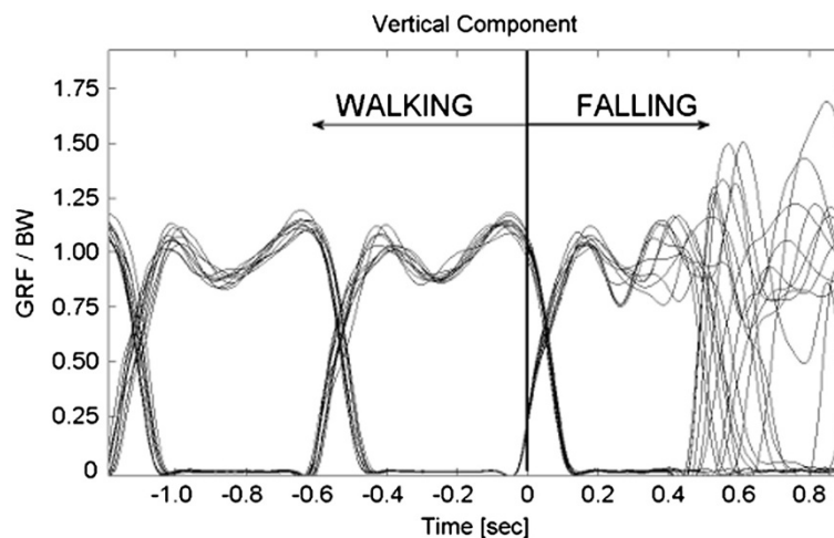
Figure 10 Vertical component of the GRF during pilot tests. GRF vertical components normalized to body weight while a subject underwent ten different perturbations occurring during the early stance phase. Walking speed was 1.11 m/s. In order to show the robustness of the algorithm triggering a specific event, all variables are aligned with respect to the trigger (Time=0).
