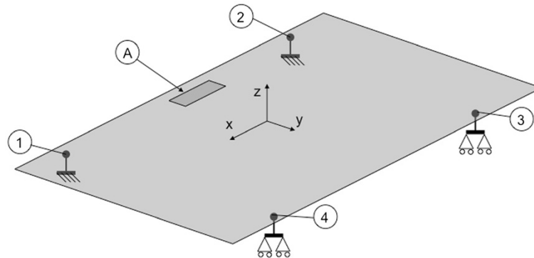
Figure 2 Schematic representation of sensorized surface related constraints. The figure shows the location of load cells on the right sensorized surface. The three-axial load cells (1, 2) are fixed to the ground (cylindrical rails) and each of the mono axial cells (3, 4) is connected to the frame by a two degrees of freedom free rail system. All tips of the load cells are connected to the sensorized surface by spherical joints. Areas A represent the rectangular extent where the load was applied during the FEA. In particular, A represents the area used by a subject while walking across both treadmills.
