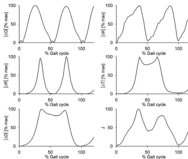
Figure 1 Example of the time patterns of the "energy-like" indices used to describe the mechanical state of the system during one gait trial. The data along the abscissa are normalised with respect to the duration of the first stride, determined as \hat{T} = \hat{t}_e - t_b .
