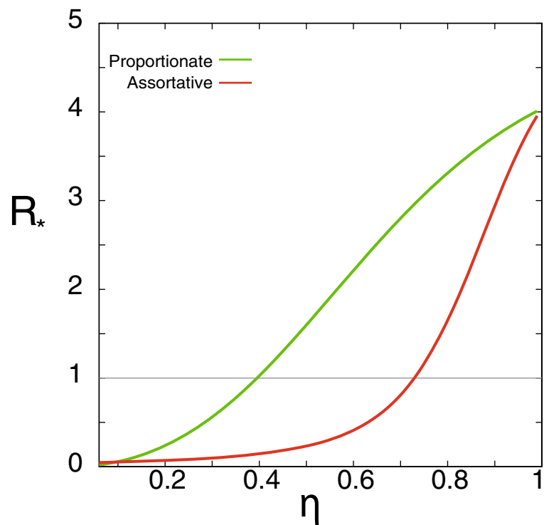
Figure 5 Comparison between proportionate and assortative social system. R_* as function of \eta for the proportionate case and the assortative one with \epsilon = 0.05 . All the other parameters are kept the same in the two curves: r = 0, \alpha = 0.4, R_0 = 1.2, \mu = 0.5, \gamma = 2.3 and w_0 = 0.05 .
