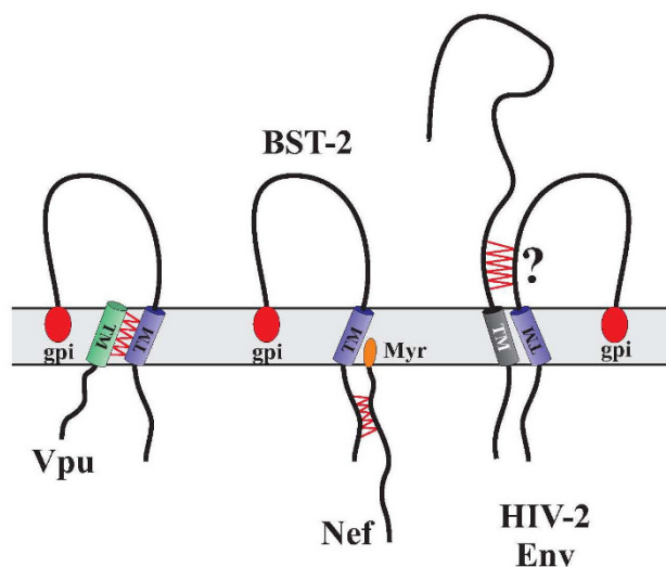
Figure 2 Interaction of BST-2 with HIV-1 proteins. Vpu interacts with BST-2 through its transmembrane domain. Interaction of BST-2 with Nef involves the cytoplasmic domain. The interaction of HIV-2 Env with BST-2 has not been mapped, but may involve the ectodomain. Proposed interaction points are indicated by red zig-zag lines. Myr: Nef myristoylation; gpi: glycosyl-phosphatidylinositol anchor.
