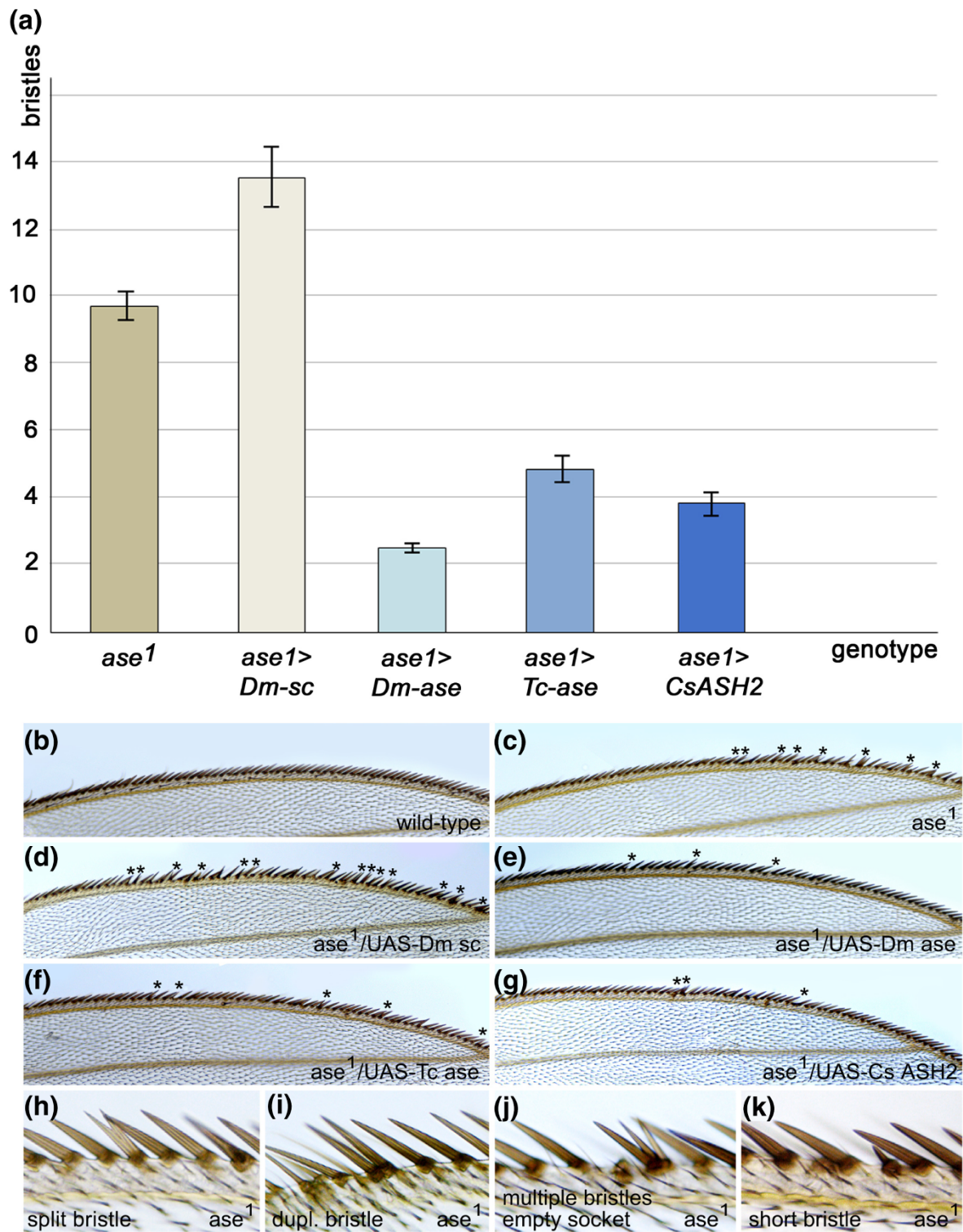
Figure 3 C. salei CsASH2 and T. castaneum ase can both rescue the bristle phenotype in D. melanogaster ase 1 mutants. (A) Bar chart showing the extent to which Dm-ase , Tc-ase and CsASH2 can rescue the phenotype when ectopically expressed ( hsp70Gal4 > UAS Dm-sc/Dm-ase/Tc-ase/CsASH2 ). In contrast, Dm-sc enhances the ase 1 phenotype ( hsp70Gal4 > UAS Dm-sc ). The number of bristles affected is given on the x-axis. Error bars indicate the standard error of the mean (see Additional file 1 for details). (B-G) Abnormally differentiated bristles (asterisks) on the anterior wing margin are shown for the genotypes indicated (genotypes as in (A)). The number of abnormal bristles is enhanced in (D) and reduced in (F, E, G). (H-K) Detail of the abnormalities at higher magnification.
