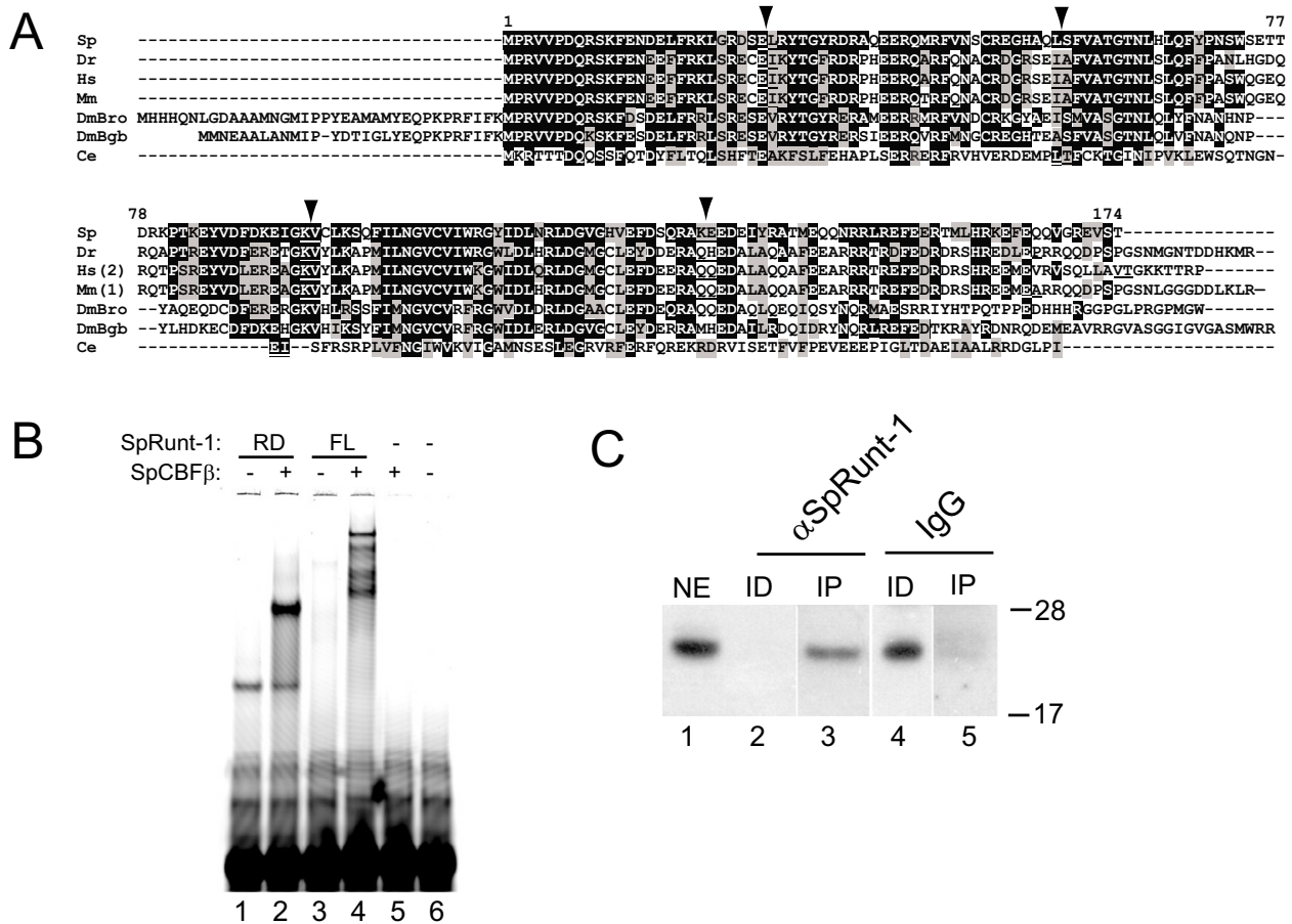
Figure 1 SpCBFβ structure and heterodimerization with SpRunt-1. (A) Alignment of CBFβ sequences from S. purpuratus (Sp) zebrafish (Dr), Homo sapiens (Hs, variant 2 of the two mammalian splice variants), mouse (Mm, variant 1 of the two mammalian splice variants), Drosophila (two genes, DmBro and DmBgb), and C. elegans . Amino acid residues that are identical between SpCBFβ and at least one other homologue are highlighted in black, and conserved substitutions are highlighted in grey. Amino acid pairs of which the respective codons are separated by introns in each gene are underlined; the four introns conserved between urchin and vertebrates are indicated by arrowheads. (B) EMSA analysis using recombinant Runt domain (RD) or full-length SpRunt-1 (FL) either alone or in the presence of recombinant SpCBFβ. Note that the full-length SpRunt-1 does not bind DNA very effectively by itself, suggesting the presence of domains that inhibit DNA binding within the full length protein. SpCBFβ complexes with both the Runt domain and full-length SpRunt-1, as indicated by a “supershift”, but does not bind DNA by itself. (C) Immunoblot of SpCBFβ from nuclear extract (NE), and nuclear extract immunodepleted (ID) and immunoprecipitated (IP) with anti-SpRunt-1 or nonspecific IgG. Molecular weight markers (in kilodaltons) are shown on the right.
