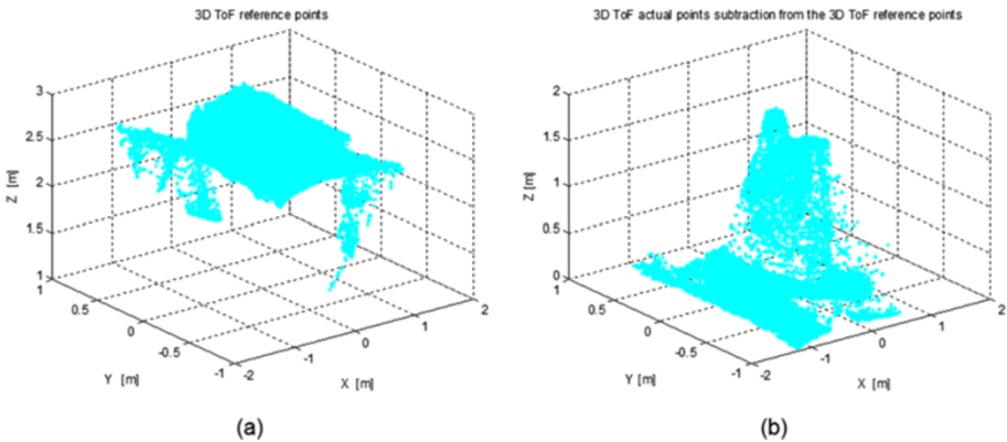
Figure 11 Foreground detection of 3D points expressed in ToF camera frame. (a) Background reference matrix B'_T to be used in foreground detection of 3D ToF points. (b) Value absolute of the difference image Z'_d between the reference, B'_T , and a current image Z'_c .
