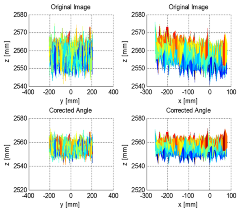
Figure 5 3D point cloud before and after angle correction. Initial 3D point cloud before and after angle correction. 3D point cloud are presented in (x, z) coordinates and in (y, z) coordinates.
