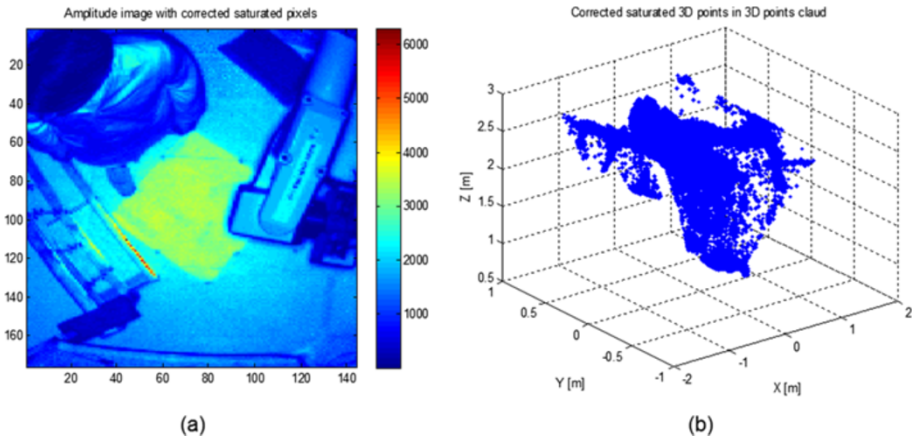
Figure 10 Saturated pixels in 3D ToF points. (a) The same amplitude ToF image is presented after pixel saturation reduction. (b) 3D ToF points after pixel saturation reduction.
