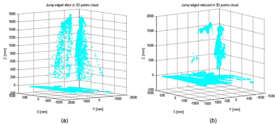
Figure 15 View of jump edge error in 3D ToF points. (a) View of 3D ToF points from the scene presented in Figure 9 in which jump edge effect appears. (b) View of the same 3D scene in which jump edge has been reduced using the morphological gradient operation.
