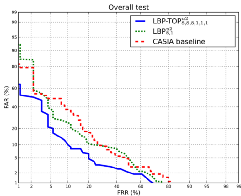
Figure 13 Overall test protocol on the CASIA Face Anti-Spoofing Database. Overall performance of LBP-TOP_{8,8,8,1,1,1}^{u2} using the average of features compared to the DoG baseline method and LBP_{8,1}^{u2} .
