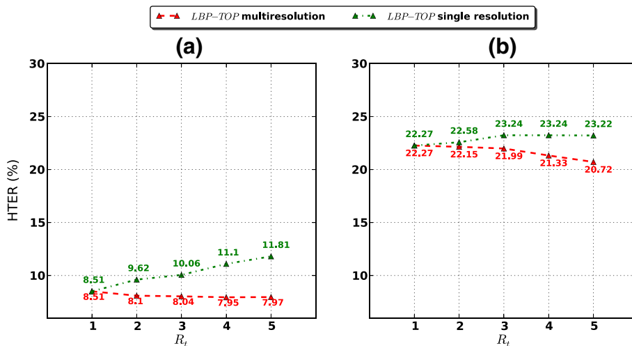
Figure 11 Evaluation of HTER (%) using LBP-TOP^{u2}_{8,8,8,1,1,R_t} with single resolution and multiresolution approach using SVM classifier. (a) Replay-Attack Database. (b) CASIA Face Anti-Spoofing database.
