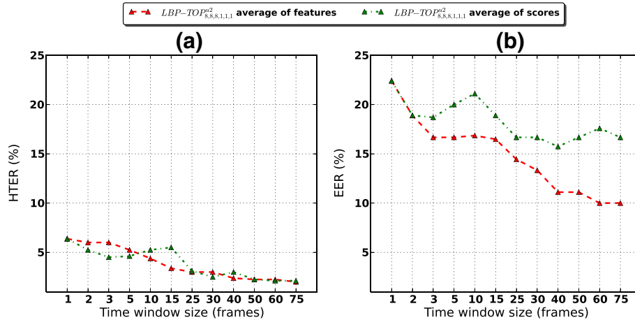
Figure 12 Access attempt-based evaluation. Different time window sizes were evaluated using mean of features and mean of scores with LBP-TOP_{8,8,8,1,1,1}^{u2} . (a) Replay-Attack Database (HTER %). (b) CASIA Face Anti-Spoofing Database (EER %).
