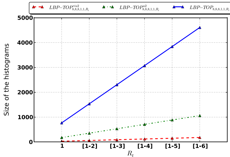
Figure 10 Evaluation of the histogram size when ( R_t ) is increased.
