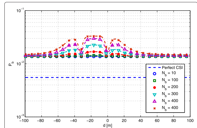
Figure 19 BER as a function of distance to the cluster. With respect to R_x and a frame length N_b at the rate SNR = 10 db and three pilot-based estimation, V2V scenario.
