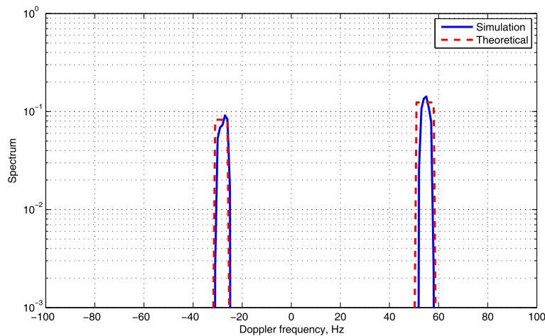
Figure 7 Doppler PSD of two-cluster channel, f_{D_1} \approx 55.7 Hz, f_{D_2} \approx -27.8 Hz.
