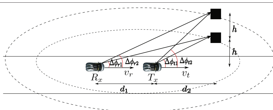
Figure 16 V2V scenario with two clusters.
