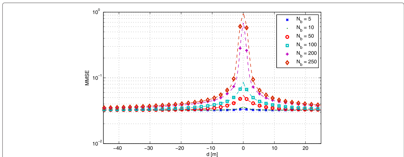
Figure 14 Estimation MMSE as a function of distance to the cluster and frame length. At SNR = 10 dB, 50 Kbps rate and three pilot-based estimation, V2I scenario.
