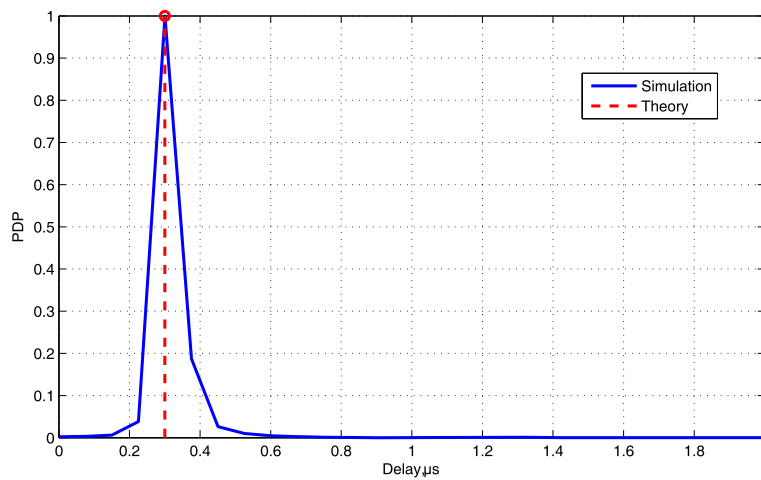
Figure 3 PDP of one-cluster channel response, \tau = 0.3 \mu\text{s} .
