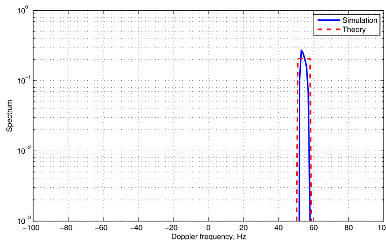
Figure 4 Doppler PSD of one-cluster channel response, f_D \approx 54.7 \text{ Hz} .
