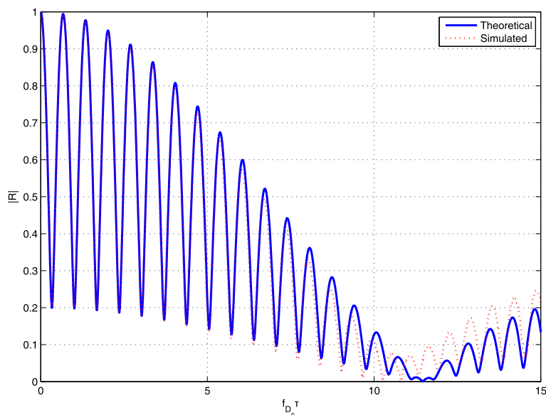
Figure 8 Envelope of auto-covariance function of two-cluster channel process, |R(\tau)| .
