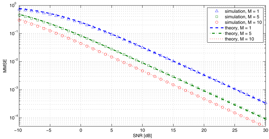
Figure 11 Estimation quality as a function of SNR and number of pilot signals M .
