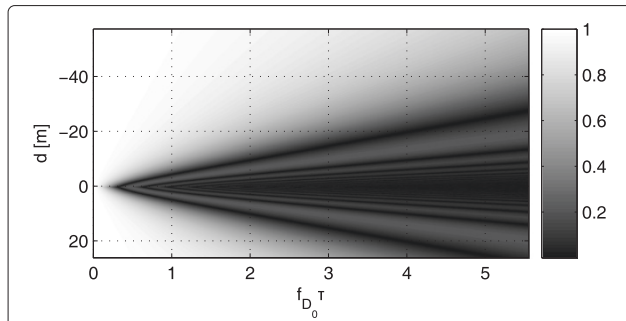
Figure 13 Absolute value of autocorrelation function of channel gains, |R(d, f_{D_0}, \tau)| , V2I scenario.
