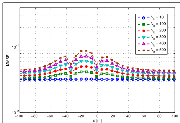
Figure 18 Estimation MMSE as a function of distance to the cluster. With respect to R_x and a frame length N_b at SNR = 10 db and three pilot-based estimation, V2V scenario.
