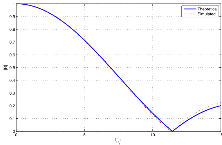
Figure 5 Envelope of the auto-covariance function of the channel process, |R(\tau)| .
