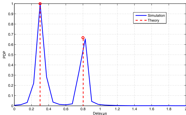
Figure 6 PDP of a two-cluster case, \tau_1 = 0.3 \mu\text{s}, \tau_2 = 0.8 \mu\text{s} .
