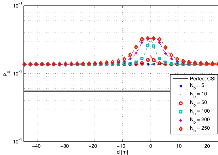
Figure 15 BER as a function of distance to the cluster. At SNR = 10 dB, 50 Kbps rate and three pilot-based estimation, V2I scenario.
