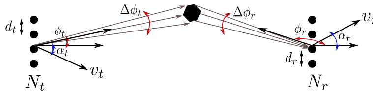
Figure 1 Geometry of a single cluster problem.
