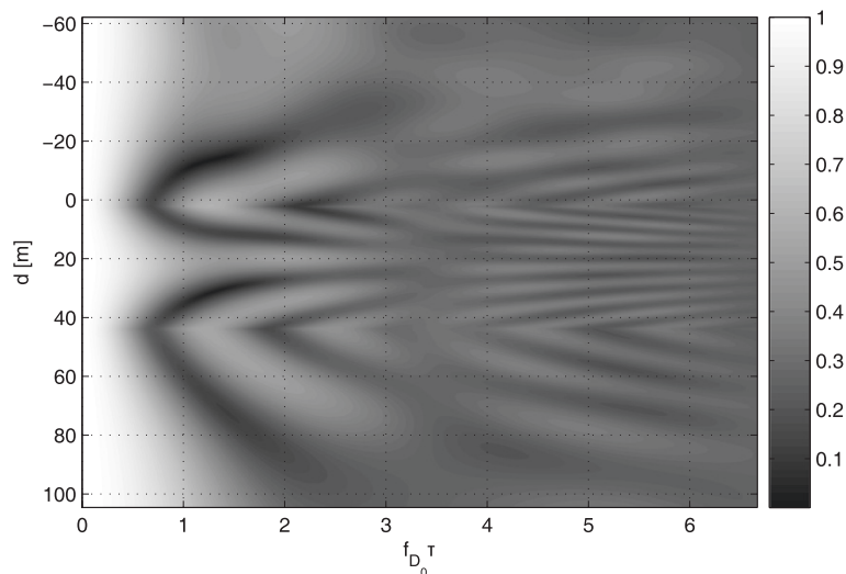
Figure 24 Auto-correlation function in a real-life scenario, Oxford Street - Wonderland Road intersection, London, ON, Canada.
