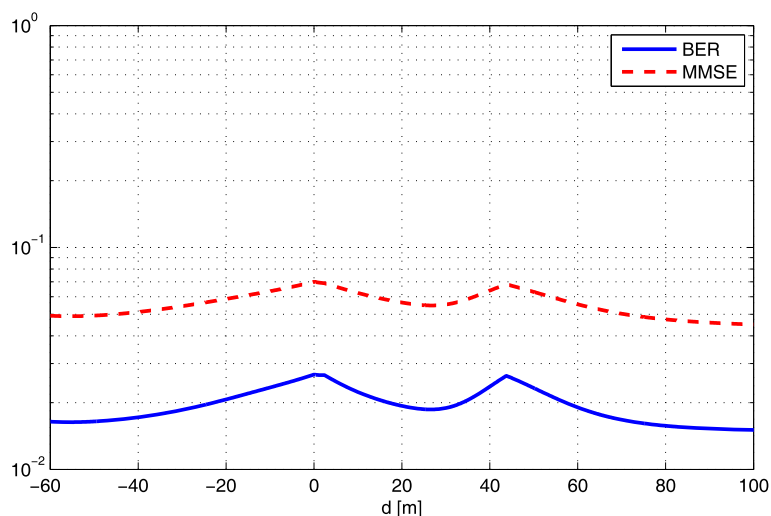
Figure 25 MMSE and BER as functions of distance to the cluster, Oxford Street - Wonderland Road intersection, London, ON, Canada.
