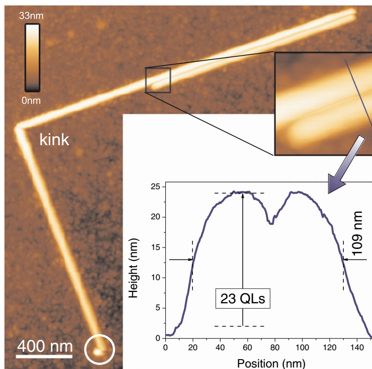
Figure 4 AFM micrographs of Bi 2 Se 2 Te nanowires on Si. Two nanowires are visible which stick together side by side, having a diameter (height) of 22.0 nm or 23 quintuple layers (QLs).
