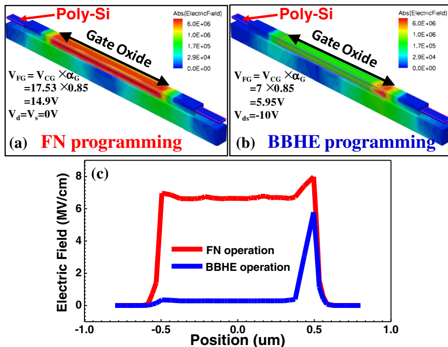
Figure 5 TCAD simulation. (a) FN programming. V_{FG} = V_{CG} \times \alpha_G = 14.9 \text{ V} . (b) BBHE programming. V_{FG} = V_{CG} \times \alpha_G = 5.95 \text{ V} . Both use the same voltage drop. (c) Electric field comparison of FN and BBHE programming.
