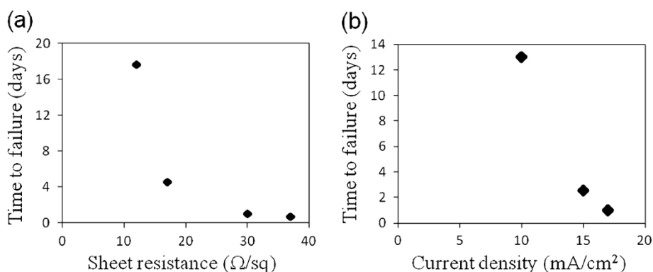
Figure 2 Dependency of failure time on resistance and current density. (a) The number of days to failure versus sheet resistance, when conducting 17 mA/cm 2 across samples with different resistances. (b) The relationship between the number of days to failure and current density, as measured with three different 30 Ω/sq electrodes.
