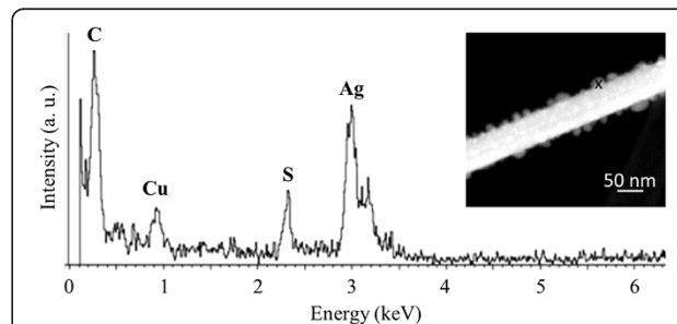
Figure 5 Energy-dispersive spectrum of a nanoparticle formed on a silver nanowire after electrode failure. The 'x' indicates the location where the measurement was taken. Sulfur was detected in the nanoparticles indicating corrosion of the silver.
