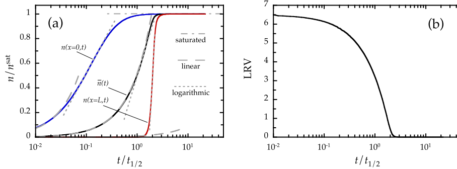
Figure 2 Time dependence. (a) Results, obtained by integrating Equations 5 to 7, for the time dependence of the areal density of trapped impurities (continuous lines) at the entrance of the channel n(x = 0, t) and at its exit point n(x = L, t) , and also the global average areal density of trapped impurities \bar{n}(t) = L^{-1} \int_0^L n(x, t) dx . The areal density axis is normalized by the saturation value n^{\text{sat}} . The time axis is normalized by the half-saturation time, defined by \bar{n}(t_{1/2}) = n^{\text{sat}}/2 . The parameter values used are as follows (see main text for details): \rho_0 = 13 nm, \rho_1 = 0.11 , \lambda_D = 5.1 nm, n^{\text{sat}} = 1.5 \times 10^{15}/\text{m}^2 = 0.25/\rho_0^2 , r_0 = 500 nm, r_1 = 8.8 \times 10^{-24} , \text{m}^3 = 4\rho_0^3 , \Omega_0 = 0 , \Omega_1 z_0 = 1.2 \times 10^5/\text{m} , L = 7.25 mm, P = 3 \times 10^5 Pa, \eta = 10^{-3} Pa-s, and C_{\text{imp}}(x = 0, t) = 10^{10}/\text{m}^3 . We also show the linear, logarithmic, and saturated behaviors (as dashed, dotted, and dot-dashed lines respectively). (b) Time dependence of the logarithmic removal value (LRV), calculated using the same parameter values as in Figure 2a.
