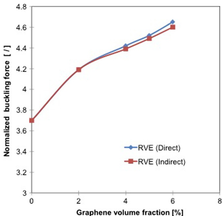
Figure 4 Normalized buckling force estimated from multiscale modeling for graphene/polymer nanocomposites. Ordinate data was normalized by dividing the critical buckling force by 10-2 nN.
