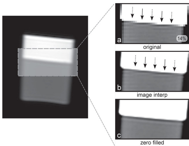
Figure 2 Phantom images. A phantom with a near horizontal flat edge between undiluted gelatine and a solution of Gd-DTPA, corresponding to a signal ratio of 1:3 in the edge boundary. a) Phantom image uninterpolated. b) Image a interpolated in the image space with a bicubic interpolation. The solid arrows point into the regions where Gibbs artifacts are visible, while the dashed arrows point into the in-between regions with no artifact. c) Image a but with zero-filling pre FFT interpolation. Figure 2 a (bottom right) shows the measured peak artifact signal loss in the bottom right corner.
