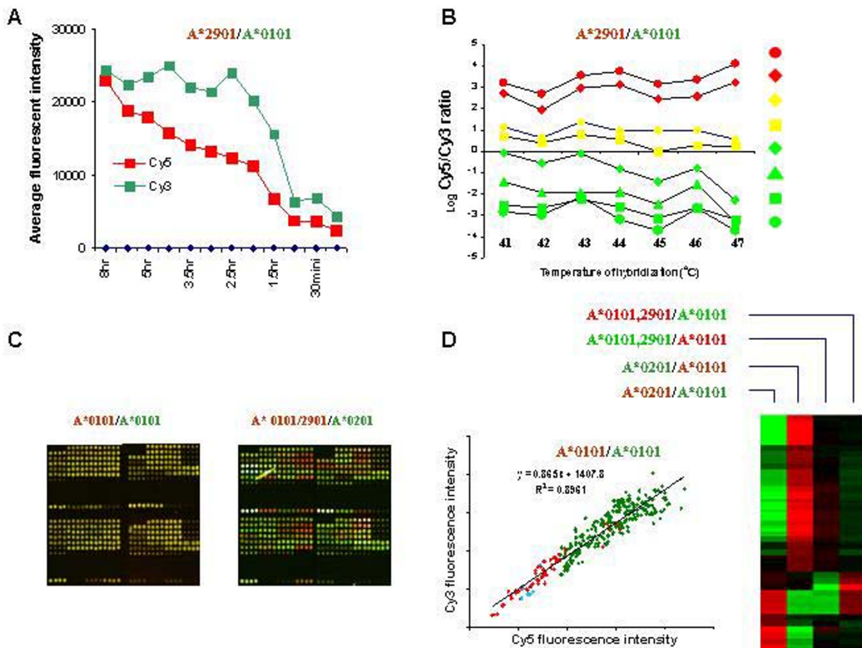
Figure 4 Effect of hybridization time (a) and temperature (b) in conditions of b,b type homozygosity (HLA-A*2901 labeled with Cy5 vs HLA-A*0101 labeled with Cy3). b ) \log Ratio for Va (HLA-A*2901-specific) oligos (red), k -oligos (yellow) and CO-oligos. c ) Test for labeling bias and reproducibility in conditions of a,a homozygosity and b,c heterozygosity: gene pix image. d ) Scatter plot of Cy3 and Cy5 fluorescence intensity in conditions of a,a homozygosity. In red are portrayed Va oligos; in green k and consensus oligos. A cluster of consensus oligos with poor hybridization kinetics due to high CG content (average of 75%) is portrayed in light blue. Reproducibility was tested in conditions of b,b homozygosity (HLA-A*0201 vs HLA-A*0101) and a,b heterozygosity (HLA-A*0101, 2901 vs HLA-A*0101) by reciprocally labeling test and reference targets in duplicate experiments as shown by the clusterogram. In spite of variable hybridization kinetics, differential hybridization could be observed consistently among Va and corresponding consensus oligos. Only HLA-A*0201-specific and relevant homologous consensus oligos (solid red and green bar respectively) or HLA-A*2901-specific oligos (dashed red line) are shown.
