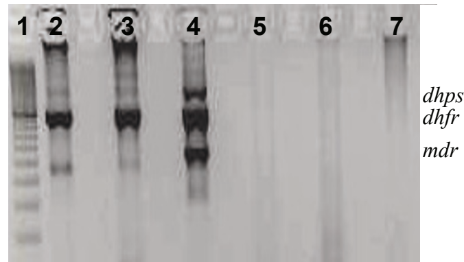
Figure 1 Gel picture after nested multiplex amplification of pvdhfr , pvdhps and pvmdr1 fragments. 1: 100 bp DNA ladder. 2: P. vivax infected monkey blood (Thai 3). 3 P. vivax infected monkey blood (Sal1). 4: P. vivax positive PNG isolate. 5: P. falciparum 3d7. 6: Human DNA ( Plasmodium sp negative). 7: Blank (water).
