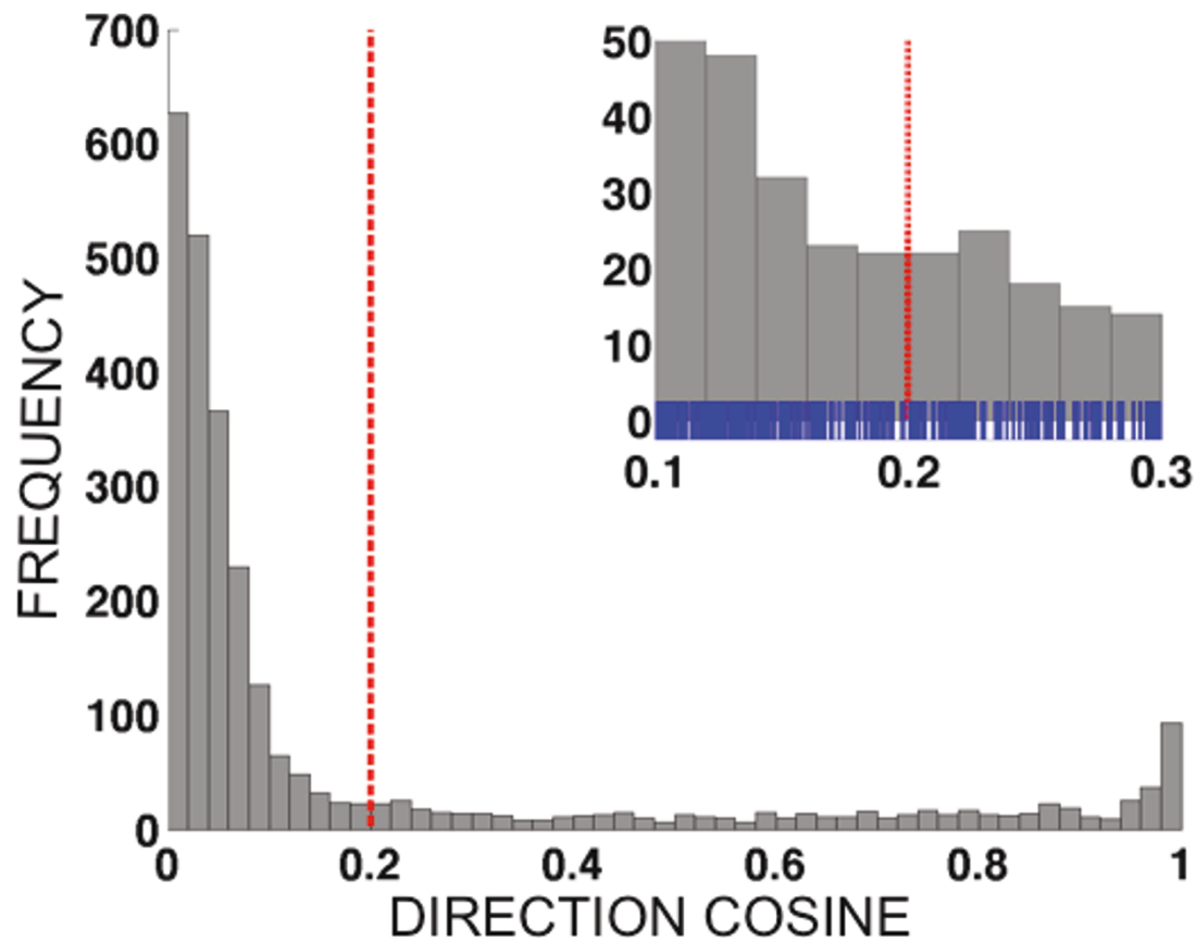
Figure 4 Histograms showing the distribution of all N_{inf} \times n direction cosine values, \{\alpha_{ij}; 1 \leq i \leq N_{inf}, 1 \leq j \leq n\} for different multi-allelic data sets. Only samples judged to be infected based on the magnitude histogram (see Figure 1) are included; the number of infected samples is denoted N_{inf} , and the number of alleles for a given data set is denoted n . The dashed vertical line indicates the diagnosis threshold for infection vs. noninfection of individual alleles. For the multi-allelic data sets, the thresholds were determined by visual inspection of the histograms. The pvdhfr 57-58-61 data contained eight alleles, giving 338 \times 8 = 2704 direction cosines total in the histogram; direction cosine threshold = 0.2. Histogram bin width = 0.02. Inset panel shows magnified region near the diagnostic threshold, including small vertical blue tick marks indicating the direction cosines for individual alleles. Corresponding figures for pvdhps 382-383 (with four alleles) and for pvdhfr 117 (with three alleles) are available as Figures S2 and S4, respectively (See Additional Files 4 and 5).
