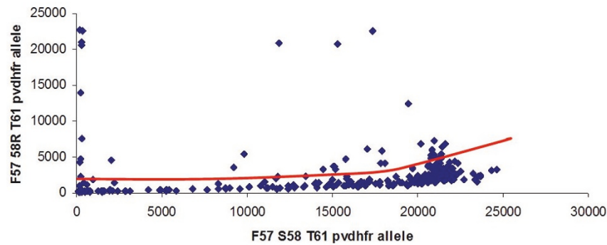
Figure 2 Increase of the allele-specific background (F57 58R T61 allele signal) observed proportionally to the intensity of another allele-specific signal (F57 S58 T61 allele signal).
