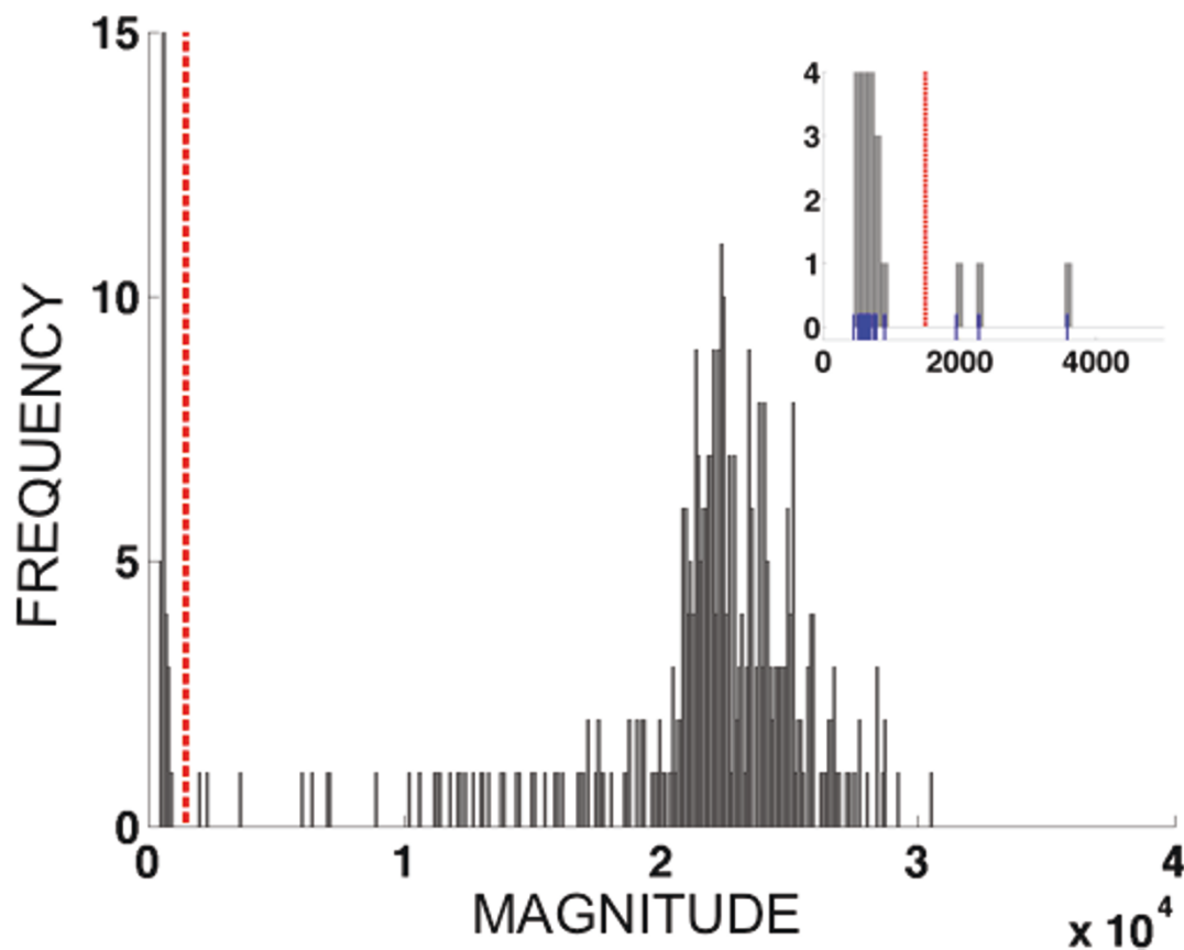
Figure 3 Histogram showing the distribution of fluorescence vector lengths \{L_i; 1 \leq i \leq N\} for a multi-allelic data set ( pvdhfr 57-58-61, eight alleles). The dashed vertical line indicates the diagnosis threshold for infection vs. noninfection. Magnitude threshold = 1500; N_{inf} = 338 . Histogram bin width = 100 fluorescence units. Inset panel shows magnified region near the diagnostic threshold, including small vertical blue tick marks indicating the magnitudes for individual samples. Corresponding figures for pvdhps 382-383 (with four alleles) and for pvdhfr 117 (with three alleles) are available as Figures S1 and S3, respectively (See Additional Files 4 and 5).
