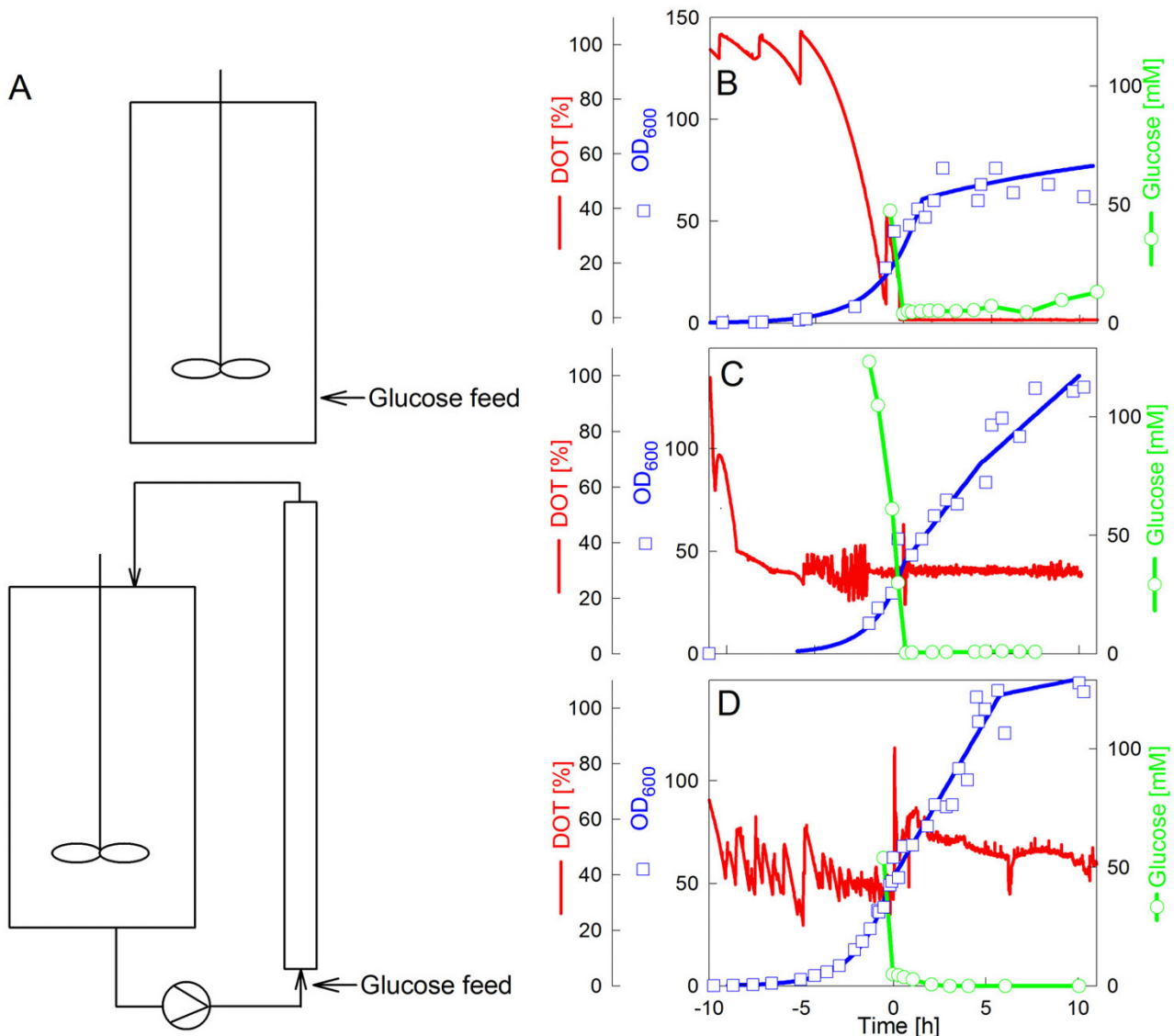
Presentation of different cultivation modes used in this study. (A) Scheme of the two reactor setups used in the study, a standard fed-batch in a stirred tank reactor and a fed-batch performed in a STR-PFR two-compartment reactor system with feeding of the glucose feed solution into the entrance of the PFR. (B-D) illustrate typical cultivation data of E. coli W3110 with the different types of cultivation applied in this study. (B) Glucose limited fed-batch cultivation with continuous feed of glucose at a constant feed rate in a single STR (reference). (C) Same as (B) but with a downshift of the DOT by a simultaneous decrease of stirrer speed and aeration rate. (D) Cultivation in a STR-PFR system with feeding of the glucose feed solution into the lower part of the PFR. The graphs show the experimental data for cell density (OD 600 ), glucose concentration, and the DOT. All analyses from the STR-PFR system were performed from samples collected by the standard sampling valve in the STR. Zero hours indicates the time of the feed start. The analyses in (C) reflect samples taken from the STR compartment. All cultivations were started with a glucose concentration of 40 g L -1 .
