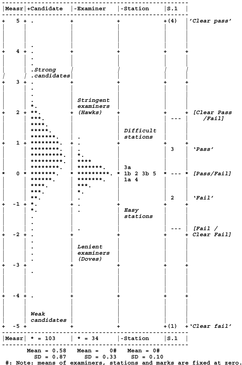
Figure 2 The 'yardstick' comparing marks on a common logit scale for candidate ability, examiner stringency, station difficulty and scaled marks.
