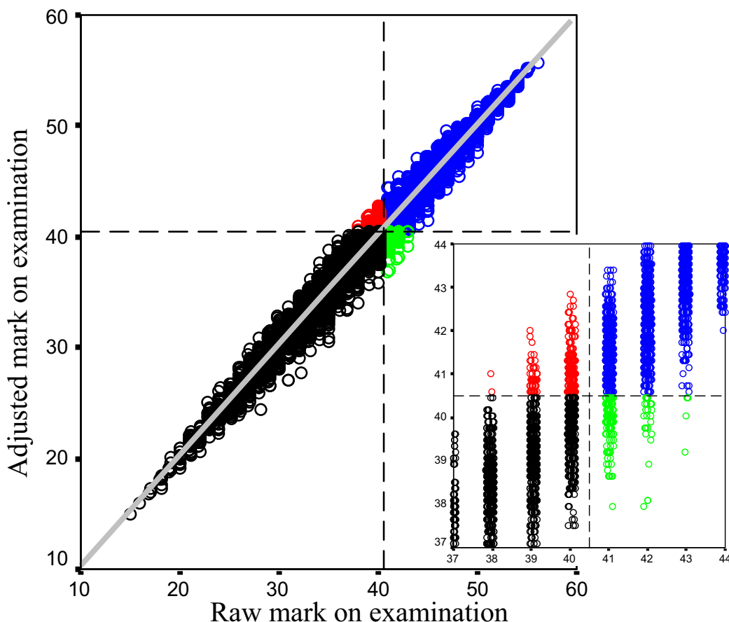
Figure 8 The relationship between the raw mark on the examination and the FACETS adjusted mark which takes examiner stringency and station difficulty into account. The pass mark for the examination is indicated by the dashed lines and has been set at 40.5 (see text; i.e. between 40 (fail) and 41 (pass)). Candidates marked in black fail the exam using both raw and adjusted marks, and candidates in blue pass the examination using both raw and adjusted marks. Candidates in green pass the exam on the basis of their raw mark but fail on the basis of the adjusted mark, and candidates in red fail on the basis of their raw mark but pass on the basis of their adjusted mark. The inset figure shows a magnification of the region around the pass mark. It should be noted that a small amount of random horizontal jitter has been applied to the raw marks (which have to be integers) so that the data points are more easily seen.
