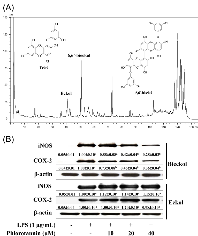
Figure 8 Identification of eckol and 6,6'-bieckol in EMM. (A) HPLC chromatogram of EMM and the chemical structures of eckol and 6,6'-bieckol (insert). (B) Cells pretreated with different concentrations of eckol or 6,6'-bieckol for 1 h were stimulated with LPS for 16 h. The expression levels of iNOS and COX-2 in cells were analyzed by Western blotting using corresponding antibodies. Relative density ratios of each protein over β-actin are shown below the blots. The results presented are representative of three independent experiments. a p < 0.05 indicates significant differences compared to the control group. b p < 0.05 indicates significant differences compared to the LPS-only treated group.
