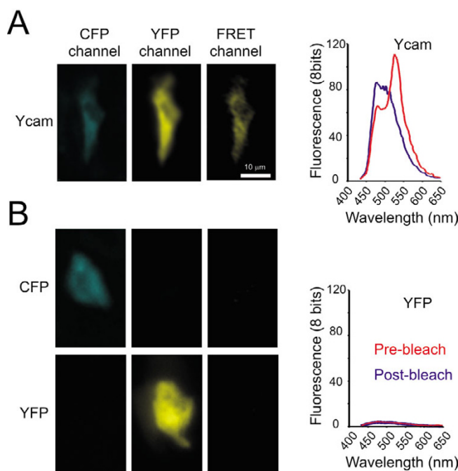
Figure 3 In vivo FRET. A) CFP, YFP and sensitized emission (FRET) images (Left panel) and emission spectra (Right panel) were collected from skin cells expressing Ycam. The red and blue spectrum are pre- and post-YFP photo destruction respectively. Note the gain in CFP fluorescence after photo destruction of YFP. B) Control experiments for intravital FRET imaging. (Left panel) The collected FRET images in A were corrected as described in methods. FRET was not observed in cells expressing only CFP or YFP, consistent with proper correction. (Right panel) The emission spectrum acquired using CFP excitation wavelength (405 nm) of a cell expressing only YFP. The expression level of YFP is similar to that of Ycam in A. Note that YFP is inefficiently excited at 405 nm, and that photo destruction of YFP does not result in an increase of fluorescence at CFP wavelengths.
