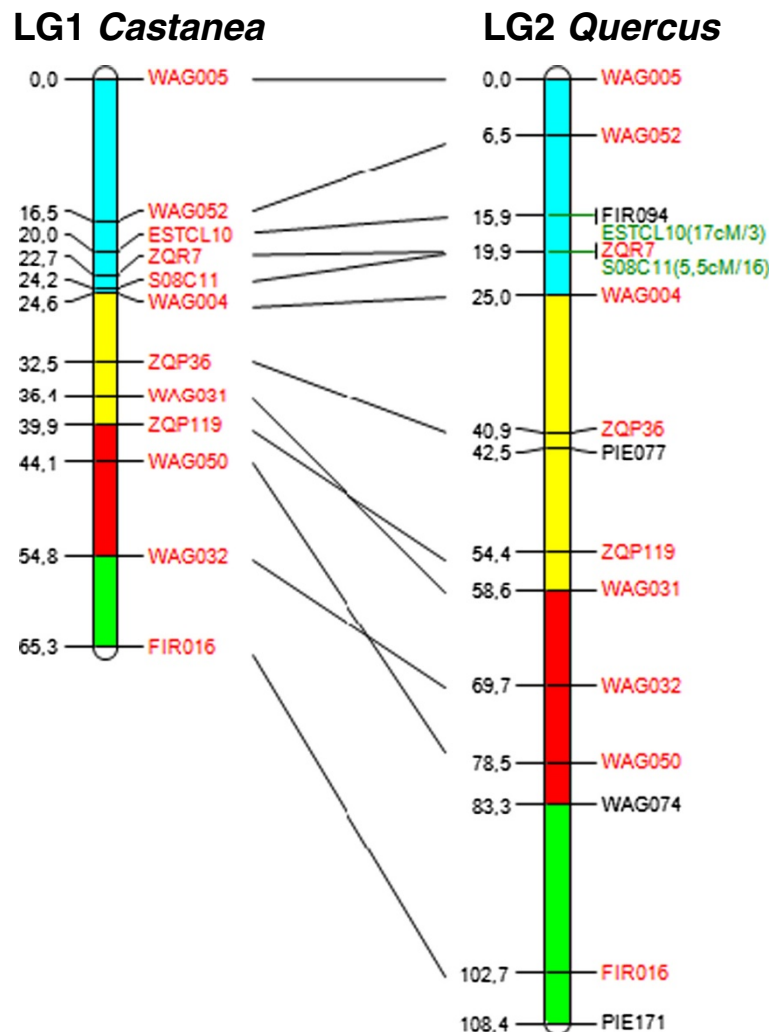
Figure 6 Synteny between Quercus and Castanea for LG1. Loci in red are common for both species, loci in green are located as accessory loci (theta/LOD), parts of linkage group which are represented by the same colour correspond to homologous segments between the two species.
