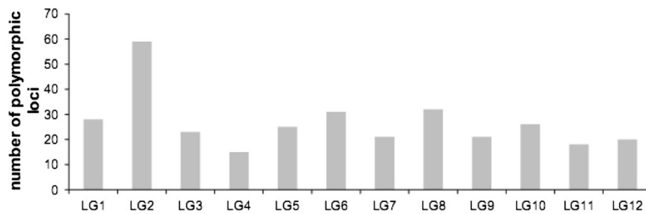
Figure 3 Distribution of common loci per LG for at least two maps.
