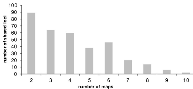
Figure 4 Number of shared loci between two to ten parental maps.
