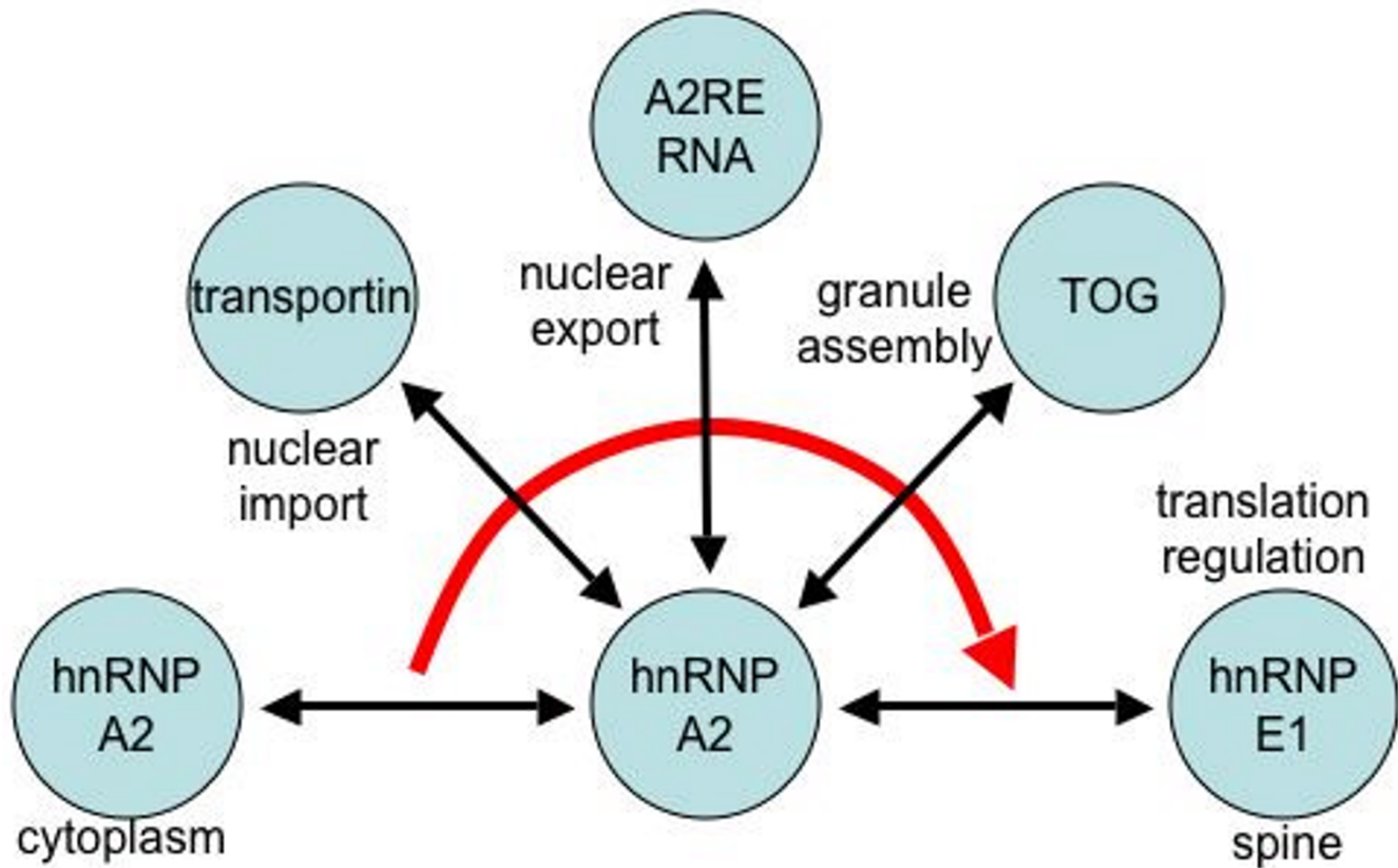
Figure 1 Molecular interactions of hnRNP A2 in the A2 RNA trafficking pathway. Five different molecular partners of hnRNP A2 have been identified in the A2 RNA trafficking pathway – hnRNP A2 itself, transportin I, A2RE RNA, TOG and hnRNP E1. Each step of the A2 RNA trafficking pathway is mediated by interaction of hnRNP A2 with a particular partner. Although interactions between hnRNP A2 and each partner are reversible, the overall pathway exhibits polarity.
