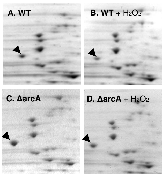
Figure 4 Two-dimensional gel electrophoresis analysis of whole cell proteins of the wild type and arcA mutant E. coli . The wild type (WT, A and B) and the arcA ( \Delta arcA , C and D) mutant E. coli were exposed to H 2 O 2 and total proteins from H 2 O 2 -exposed (+H 2 O 2 , B and D) and unexposed bacteria (A and C) were electrophoresed on 2-D gels. Arrows point to the flagellin protein.
