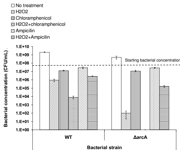
Figure 8 Chloramphenicol enhanced the bactericidal activity of H 2 O 2 . The wild type E. coli (WT) and the arcA mutant E. coli (Δ arcA ) were incubated in M9 minimal medium containing 1.5 mM H 2 O 2 for 6 hours at 37°C. The survival of bacteria was determined by plating. Bacterial concentration following each treatment (open bars, no treatment; diagonally-hatched bars, H 2 O 2 ; vertically-hatched bars, 25 µg ml -1 of chloramphenicol; cross-hatched bars, H 2 O 2 and 25 µg ml -1 of chloramphenicol; dotted line-hatched bars, 50 µg ml -1 ampicillin and horizontally-hatched bars, H 2 O 2 and 50 µg ml -1 ampicillin) was plotted on the graph. The horizontal dashed line indicates the starting concentration of bacteria.
