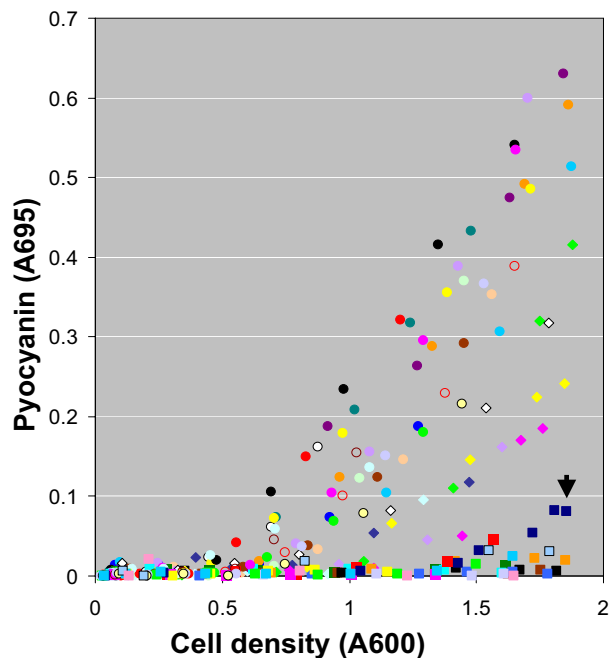
Figure 2 Pyocyanin assays on LES isolates. Production of pyocyanin in culture supernatants during growth of LES isolates in L-broth is shown for all the LES isolates tested in this study. Each combination of colour and shape plotted represents a different LES isolate. The only non-LES isolate included is strain PA01 (blue squares, indicated by the arrow). LES isolates could be sub-divided on the basis of pyocyanin assays into various groups: (i) OP (early- and over-production of pyocyanin) [circles]. (ii) Intermediate [diamonds]. (iii) Normal or negative [squares]
