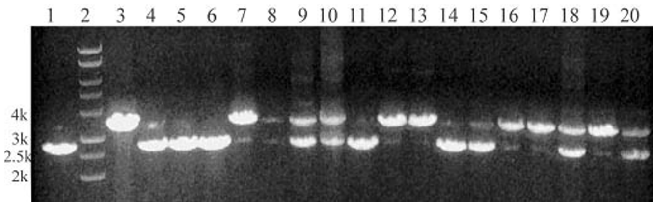
Figure 6 Colony PCR products for identifying uracil-independent transformants using genomic DNA extracted by CTAB method and primer pairs P1 and P6. Lane 1: The control native target sequence which PCR-amplified from 3357-5; Lane 3–20: From different transformant colonies.
