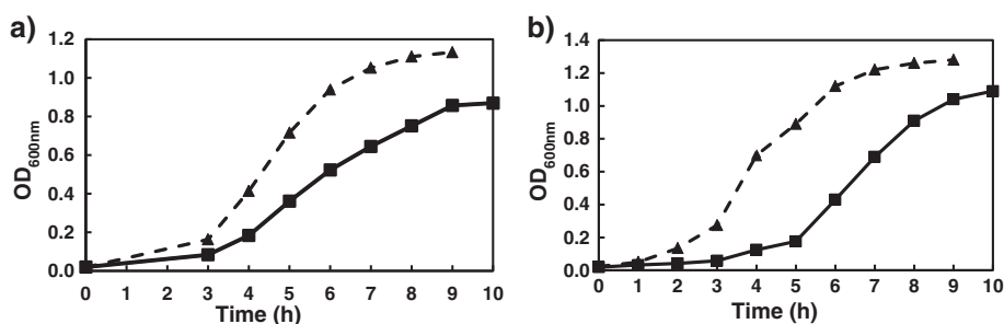
Figure 1 a) Effect of overexpression of luxR on the growth rate of V. scopthalmi . V. scopthalmi A089_23 (pMMB207) (black triangle) used as control strain vs V. scopthalmi A089_23 (pMMB207::luxR) (black square); b) Effect of expression of the lactonase aiiA in V. scopthalmi A102. The growth rate was reduced in V. scopthalmi A089_23 overexpressing luxR (black square) compared to the control strain (black triangle) (Figure 1a), while strain A102_6.2 expressing the lactonase (black square) had a longer lag phase with respect to the control strain A102_pACYC (black triangle) (Figure 1b).
