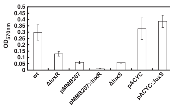
Figure 2 Biofilm formation in the V. scopthalmi A102 strain cultured in MB; wt, wild type strain; Δ luxR , A102_56 strain; Δ luxS , mutant A102_73 strain; pMMB207, A102_90; pMMB207:: luxR , A102_78 mutant; pACYC, A102_pACYC184; pACYC184:: luxS , A102_99 strain. The error bars indicate standard deviation based on three independent assays with four replicates each one. Statistical analysis was performed by student's t test. Similar results were obtained with the A089 mutant strains.
