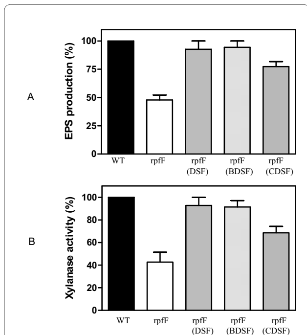
Figure 4 Effects of DSF, BDSF and CDSF on EPS production and extracellular xylanase activity of rpjF mutant of Xoo strain KACC10331. (A) EPS production at \text{OD}_{600} = 2.5 . (B) The xylanase activity in the supernatant of cell culture at \text{OD}_{600} = 2.5 . DSF, BDSF and CDSF were separately added to rpjF mutant at early growth stage at a final concentration of 3 \mu\text{M} .
