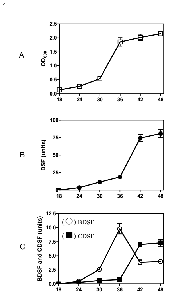
Figure 5 Time course of DSF, BDSF and CDSF production in Xoo during growth. (A) Time course of the bacterial growth in YEB medium. (B) Time course of DSF production. (C) Time course of BDSF and CDSF production. Units of DSF, BDSF and CDSF were determined by peak area in HPLC elute as indicated in Materials and Methods.
