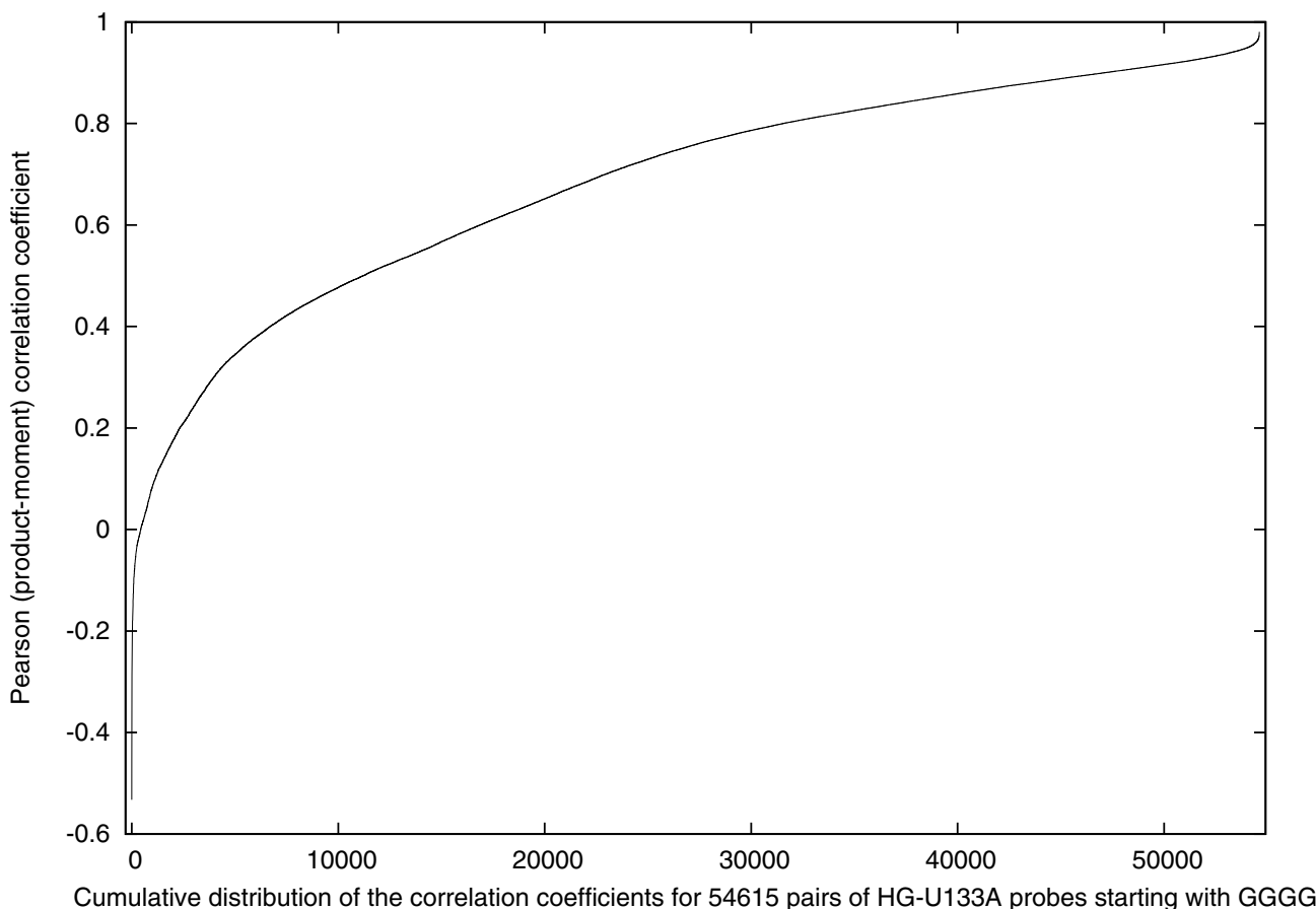
Figure 4 The distribution of the correlation coefficient for pairs of probes that begin with the sequence GGGG and contain no other runs of Gs.
