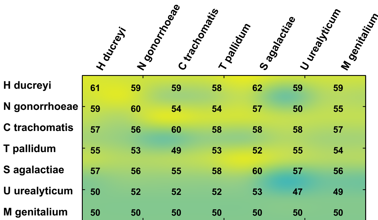
Figure 4 Classifier transfer across species boundaries. The median AUC for 13 functional classes is shown. The 'training species' is shown in the rows, the 'test' species in the columns. It can be seen that classifiers perform almost as well on a 'foreign' species as they do on the species they were originally trained on (diagonal). Performance is worst for the classifiers from T. pallidum , U. urealyticum and M. genitalium , and in these three cases the classifiers from the other four species give significantly better performance than those from the original species (sign test, p < 0.001 ).
