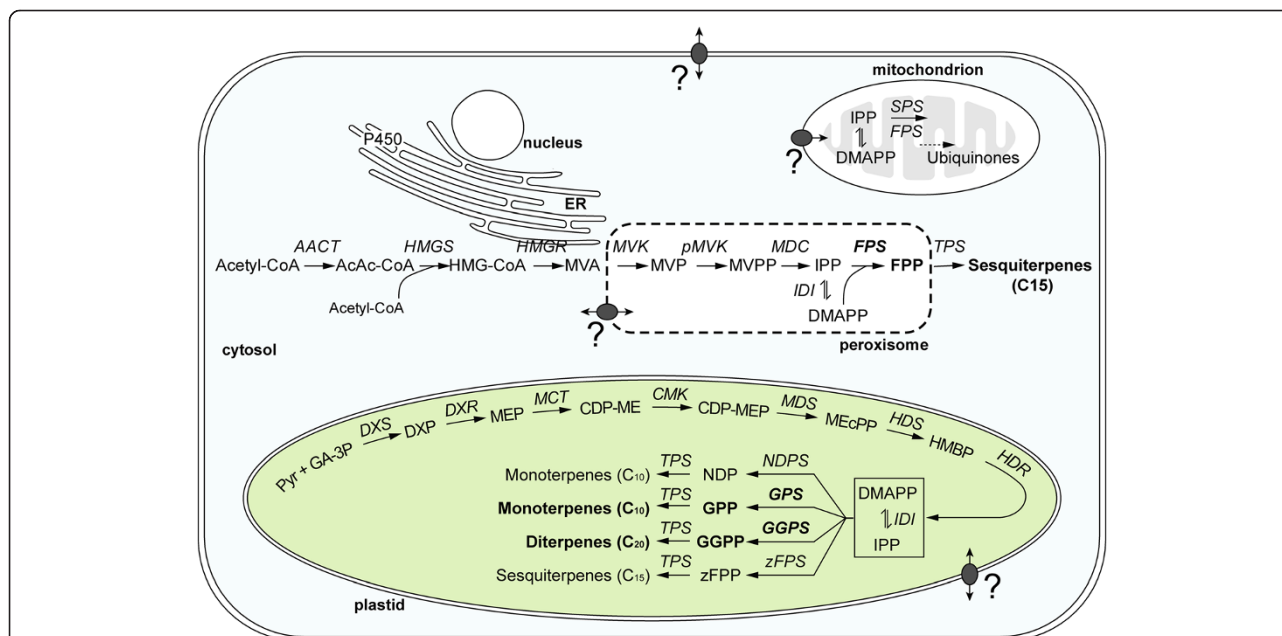
Figure 1 Enzymes involved in the precursor biosynthesis for mono-(C 10 ), sesqui-(C 15 ) and di-(C 20 ) terpenes. An explanation of the abbreviations used in the pathways and the GAll reads for each enzyme are shown in Tables 4 and 5, respectively. ER; endoplasmic reticulum, TPS; terpene synthase, SPS; solanesyl diphosphate synthase. The grey oval circles between organelles and at the cell membrane represent putative transporter systems. Peroxisomal localization of precursor enzymes of the MVA pathway has been previously reported in Arabidopsis thaliana and Catharanthus roseus [42-44].
