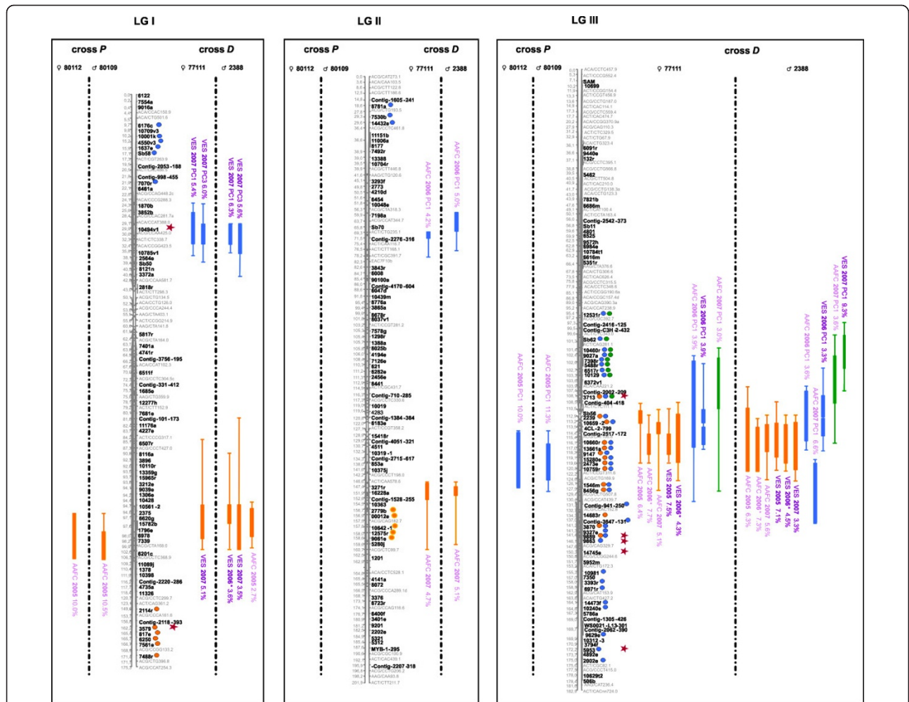
Figure 1 Genomic architecture of adaptive traits in white spruce: distribution of QTLs significantly associated to bud flush, bud set, and height growth on linkage groups I to III of the composite map of white spruce assembled from both mapping populations P (♀ 80112 × ♂ 80109) and D (♀ 77111 × ♂ 2388). Genetic distances are indicated in cM (Kosambi) at the left of each linkage group. QTLs for bud flush, bud set and height growth are indicated by green, blue, and orange circles and bars, respectively. Thin and large vertical bars of each QTL correspond respectively to -1LOD and -2LOD confidence intervals and are positioned compared to marker position on central bar of each linkage group. Circles identify gene markers associated to each -1LOD confidence interval of each QTL. Note that because of the dense positioning of markers, physical position of circles and confidence intervals can not be plotted beside each other. QTL names correspond to environmental condition (indoor = AAFC or outdoor = VES), year and for bud flush and bud set, principal component identifying each QTL, i.e. PC1, PC2 or PC3 (Table 2). An asterisk was added for QTLs identified from total height growth in order to distinguish them to QTLs identified for annual height growth in 2006 for the cross D . Red stars indicate the correspondence between QTL-marker and outlier candidate gene SNPs involved in local adaptation for white spruce [108].
