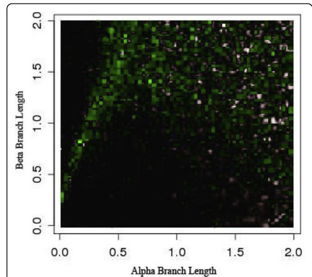
Figure 13 Parsimony vs. Likelihood using 4 taxa Comparison of Parsimony and Maximum Likelihood using a 4 taxa Felsenstein Zone tree.
