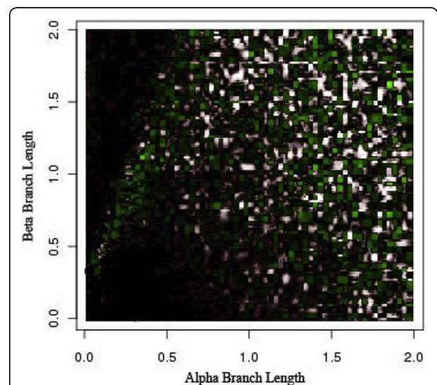
Figure 14 Parsimony vs. Likelihood using 6 taxa Comparison of Parsimony and Maximum Likelihood using a 6 taxa Felsenstein-like Zone tree.
