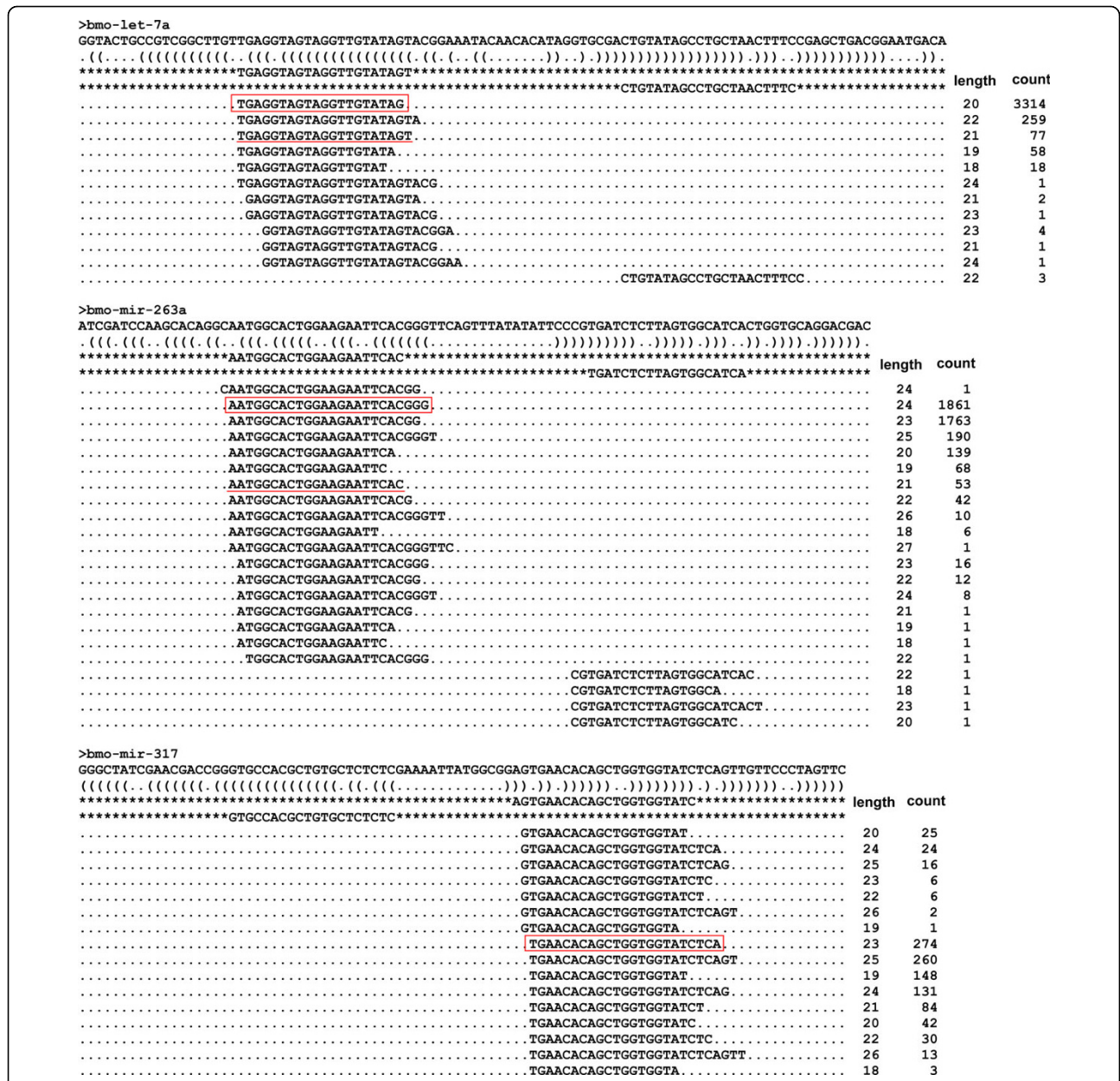
Figure 2 Heterogeneity at the 5' and 3' ends of the sequenced tags. Pre-miRNAs, structures, and multiple isoforms of expressed mature bmo-mir-263a, bmo-let-7a and bmo-mir-317 sequences and their read counts are shown. Underlined sequences are annotated in miRBase 14.0. The boxed sequences have the highest read counts. The annotated mature sequence of bmo-mir-317 was not identified, while the maximal sequence in the whole body was strongly accumulated in the two other libraries, and consequently regarded as the most active isoform.
