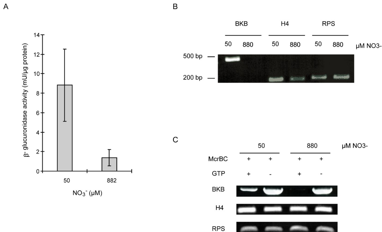
Figure 5 Regulation of Blackbeard expression. (A) Effect of nitrate limitation on the expression of the pLTRbkb-GUS-FcpA construct in transgenic P. tricornutum cells. Data represent the average with standard error from seven independent cultures after two weeks nitrate limitation (50 μM NO 3 - ) compared to standard growth medium (882 μM NO 3 - ). (B) Verification of Blackbeard transcriptional activation by semi-quantitative RT PCR in the cultures used for McrPCR. (C) McrPCR on Blackbeard and H4 and RPS controls using DNA extracted from P. tricornutum cells grown under normal and nitrate-limited conditions.
