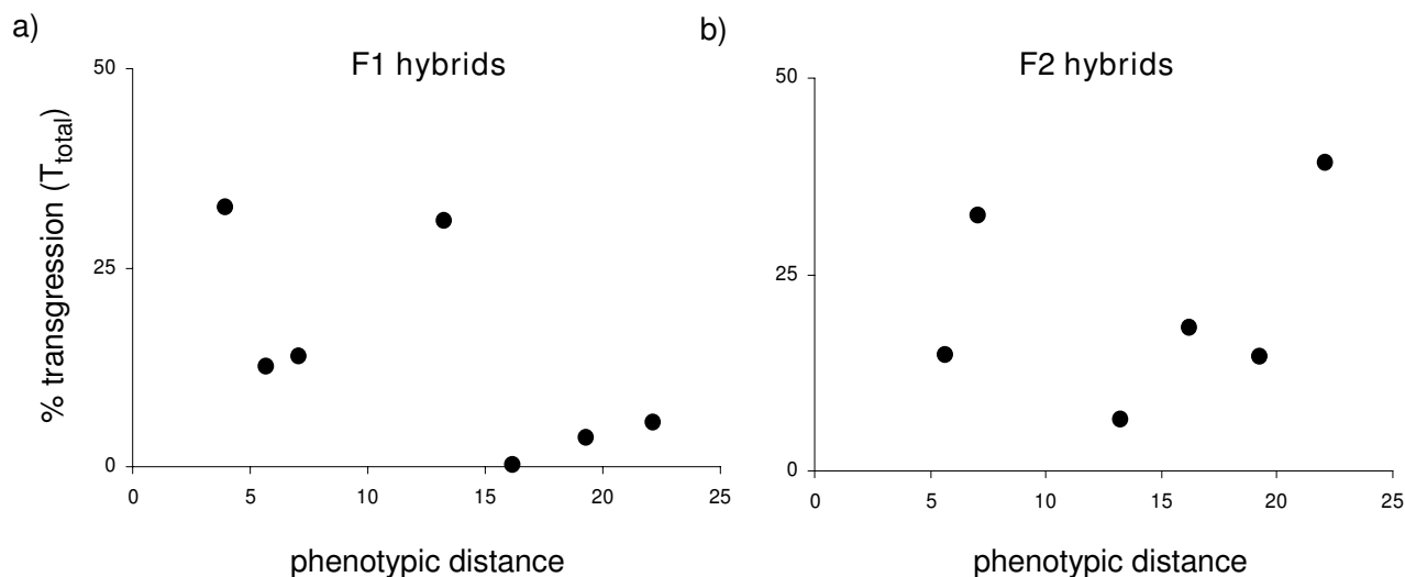
Figure 3 Total amount of transgression ( T_{total} ) observed in interspecific a) F1 hybrids and b) F2 hybrids as a function of the phenotypic distance (Mahalanobis distance calculated from 15 geometric morphometric landmarks) between the parental species. No significant relationships were found.
