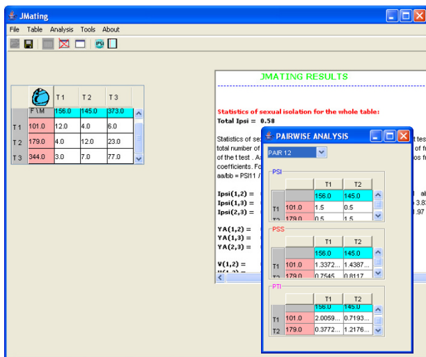
Figure 3 Example of the pairwise analysis for the mating types 1 and 2. It calculates the statistics PTI , PSI and PSS as if only data from mating types 1 (T1) and 2 (T2) were available.
