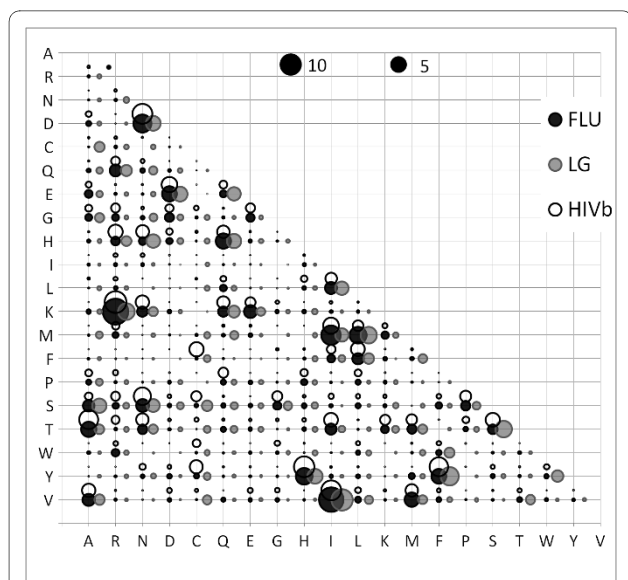
Figure 2 The exchangeability coefficients in FLU, HIVb and LG models. The black bubble at the intersection of line X and column Y presents the exchangeability between amino acid X and amino acid Y in FLU. Similarly, the grey and white bubbles present exchangeabilities between amino acids in the LG and HIVb models, respectively. These bubbles show remarkable differences between these models.
