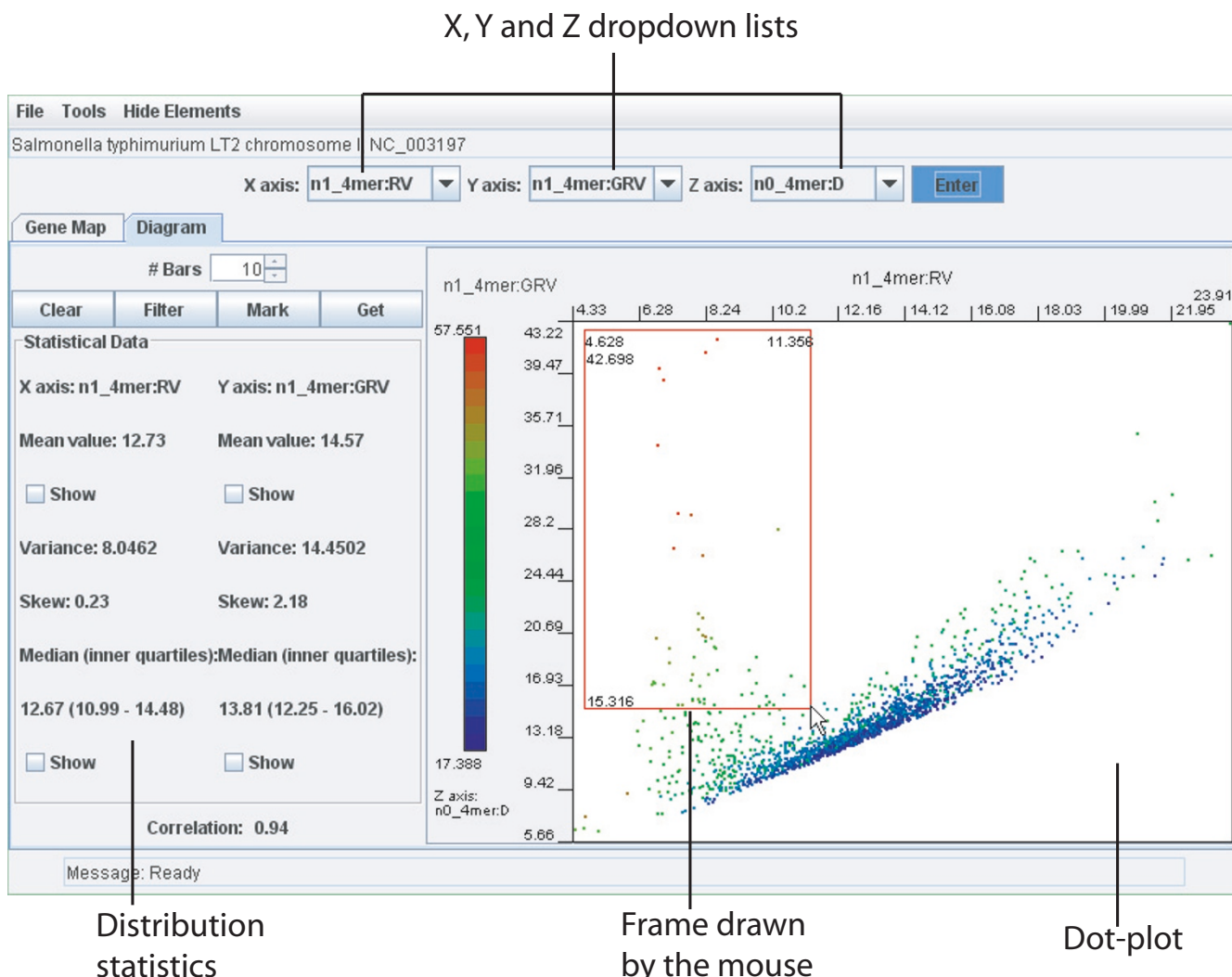
Figure 3 The 'Diagram' view. To draw a diagram, first select corresponding OU parameters using the dropdown lists and click the 'Enter' button. In this example n1_4mer:RV, n1_4mer:GRV and n0_4mer:D were selected for the X, Y and Z axes, respectively. Every dot on the dot-plot corresponds to a genomic fragment selected by the sliding window. Dots are spread and coloured in accordance with their values of the selected statistical OU parameters. Information for each dot may be found by one of the following methods: i) information for a dot under the mouse pointed by the mouse is shown in the 'Message' bar; ii) double clicking a dot returns us to the 'Gene map' tab with the corresponding genomic fragment highlighted; iii) framing the dots and clicking the 'Get' button opens a new applet window with the information about all selected regions. In this example the genomic regions of Salmonella typhimurium LT2 (NC_003197) that correspond to horizontally transferred genetic elements were selected (see discussion in the text).
