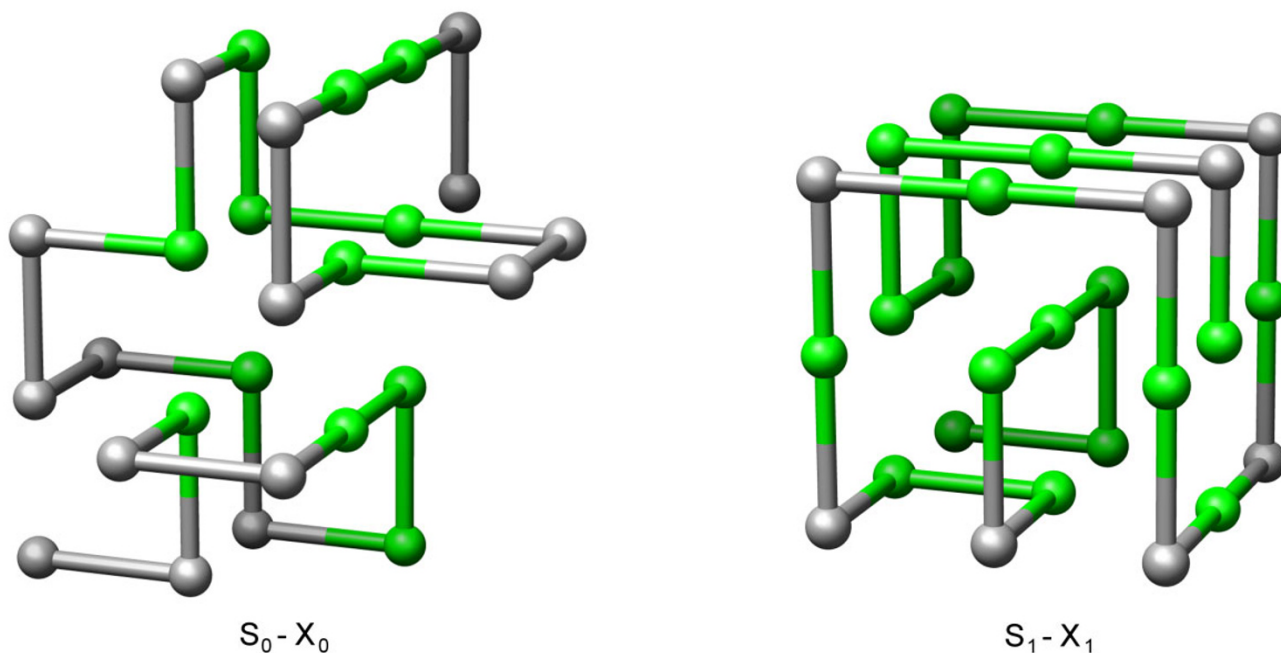
Figure 2 Structures in 3D-cubic lattice. An optimal structure X_0 for sequence S_0 and the unique optimal structure X_1 of S_1 from Table 2 in the 3D-cubic lattice. The coloring shows H-monomers in green and P-monomers in grey.
