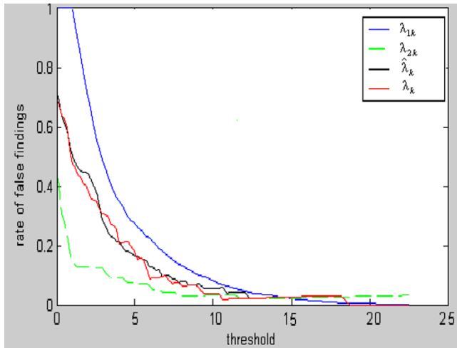
Figure 1 Profile of estimates of FDRs for a series of thresholds. \lambda_{1k} and \lambda_{2k} are two threshold functions from simulations 1 and 2 and were used to construct an estimation interval for estimate of FDR at threshold \Delta_k . \lambda_k and \hat{\lambda}_k are true and estimated FDRs at threshold \Delta_k , respectively, where k = 1, 2, \dots, L .
