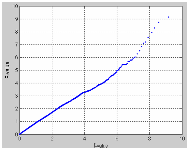
Figure 2 The dot-plot of F -values versus \bar{f} -values. F -values and \bar{f} -values obtained from the simulated microarray data of 3770 genes were ranked where \bar{f} -values were yielded by the random splitting approach. All ranked F - \bar{f} dots roughly fall on a diagonal line as expected by two sets of the same ranked distributions.
