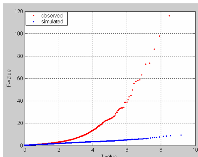
Figure 4 Comparison between the observed (red) and simulated (blue) plots of F -values versus \bar{f} -values. F -values were observed from real (red) and simulated (blue) microarray data sets of 3770 genes and 6 replicates. \bar{f} -value yielded by randomly splitting approach is an estimate in null f -distribution. F -distribution from simulated data set without treatment effects is null distribution. Ranked F -values corresponds to ranked \bar{f} -values.
