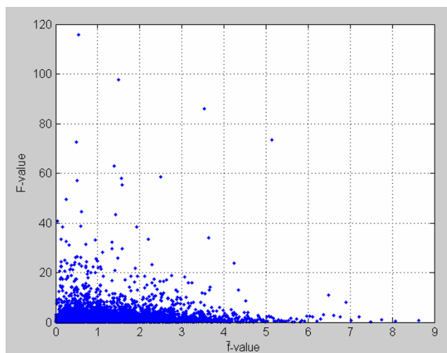
Figure 3 The scatter plot of F -values versus \bar{f} -values. F -values were observed from real microarray data set and \bar{f} -values yielded by random splitting approach are an estimate of null f -distribution.
