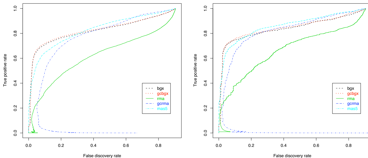
Figure 8 Performance on the Golden Spike data. Nine single-array comparisons (left) and three-replicate comparisons (right) between condition C and S were performed using BGX, GCBGX, RMA, GCRMA and MAS5. The ROC curves show that GCBGX has a small advantage over BGX and that both models perform well. For false discovery rates below 20%, BGX and GCBGX outperform RMA, GCRMA and MAS5.
