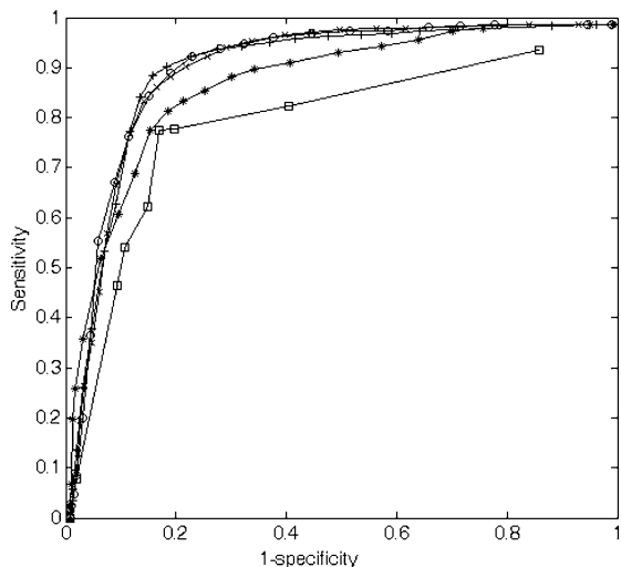
Figure 6 Changes in performance according to the numbers of features selected. The rectangle shows the ROC curve of the classifier created with the top feature, the asterisk (*) line is for the top five features, the plus symbol (+) line is for the top 10, the 'x' line is top 15, and the circle line is for the complete feature set.
