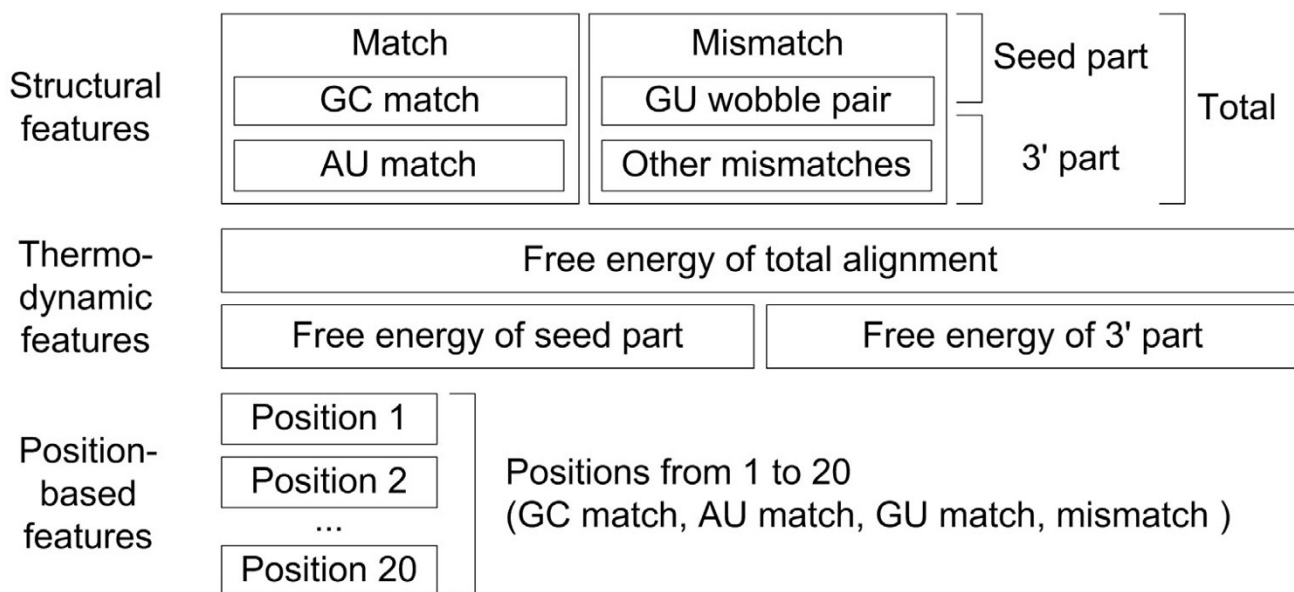
Figure 2 Three categories of SVM features.
