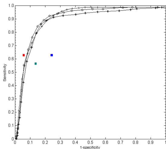
Figure 3 The ROC curves of classifiers created on three combinations of features: an entire set (circles), position-based features only (asterisks), and without position-based features (plus symbols). The red rectangle denotes the performance of TargetScan, the green one shows the performance of RNAhybrid, and the blue one shows the performance of miRanda.
