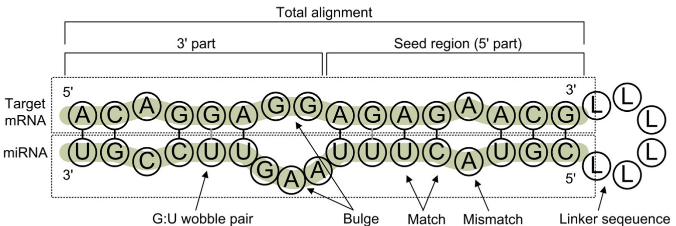
Figure 1 General scheme of miRNA:mRNA interactions.
