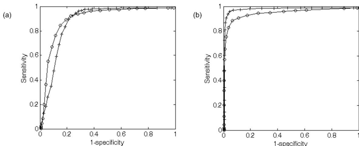
Figure 5 Comparisons between a random negative data set and an original negative data set. (a) The plots show the performance of the original (circle) and random (plus) classifiers on the original test data set. (b) The plots show the performance of the original (circle) and random (plus) classifiers on the random test data sets.
