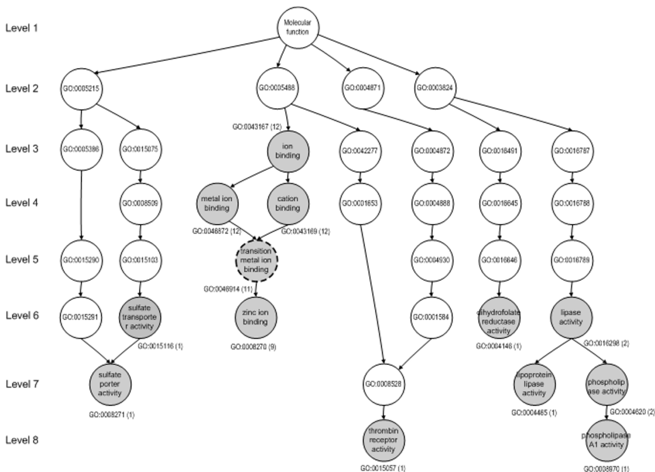
Figure 4 A subgraph of the GO-directed acyclic graph (DAG) to show functional relationships among the statistically significant GO terms for the target genes of miR-124a. The gray vertexes denote statistically significant GO terms based on a hypergeometric distribution. The numbers in brackets denote the numbers of genes annotated to the GO term. The dotted circle shows the best GO term.
