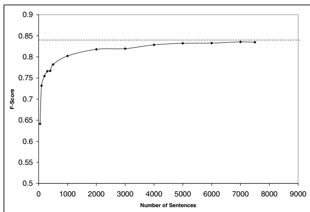
Figure 1 Learning curve. Learning curve for the performance of the "open" NER system on development data.
