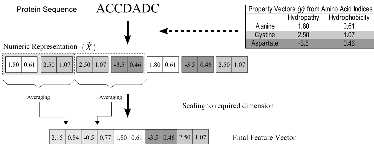
Figure 3 Feature vector construction. In this example, the physicochemical properties chosen are hydropathy and hydrophobicity . Their property vectors \{\vec{y}^i\} are concatenated in the order of occurrence of the residues in the sample protein sequence. The \vec{X} vector thus obtained is scaled by averaging to the required target dimension.
