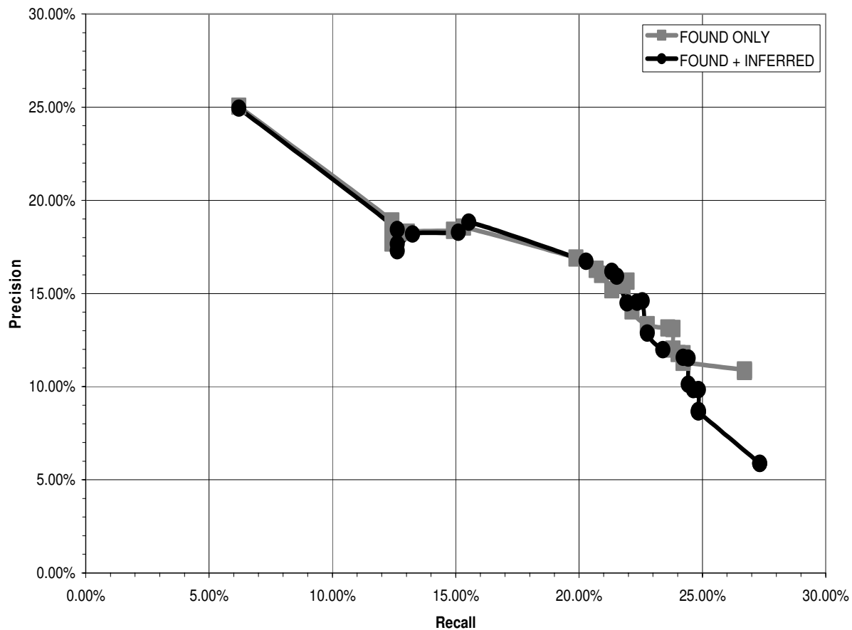
Figure 1 Precision versus recall over all iterations.
