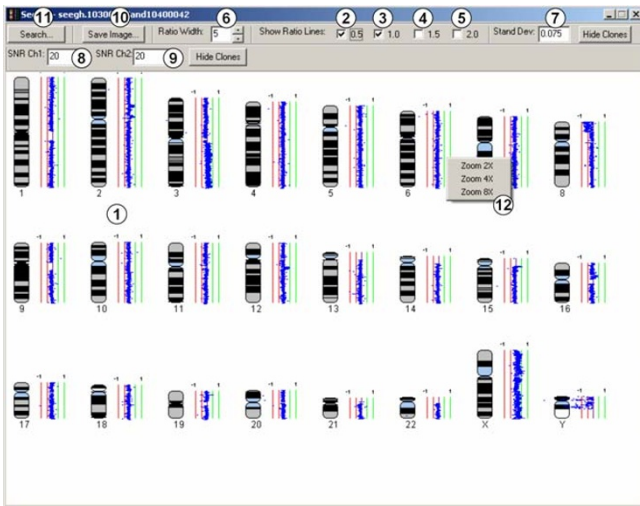
Figure 3 SeeGH "Genomic View" Window. Reconstructed whole genomic array CGH profile from 97,299 array elements. Mantle cell lymphoma DNA (labeled with Cye5) was competitively hybridized with normal male (labeled with Cye3) to an array of 32,433 DNA segments spotted in triplicate (97,299 elements). The information from the 97,299 elements was imported into SeeGH and is displayed. Buttons correspond to descriptions in the text.
