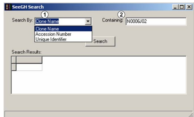
Figure 4 SeeGH "Search" Window. Buttons correspond to descriptions in the text.
