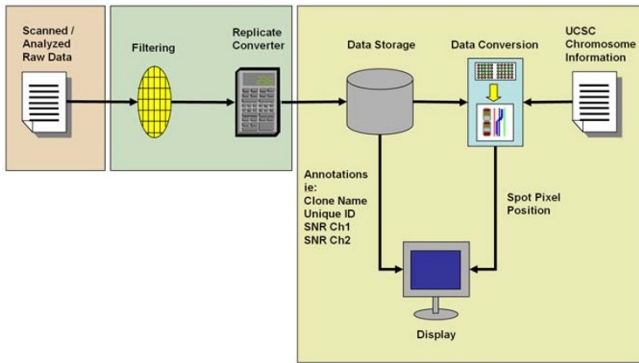
Figure 1 Overall View of SeeGH Data Flow: The user inputs data formatted as a tab delimited text file. The relevant data is then extracted from the text file via a filtering algorithm and replicate ratios and features are averaged before being stored in an SQL database. Ratio data is displayed via a data converter which converts ratio data to x, y plot coordinates, whereas annotation information is read directly from the SQL database.
