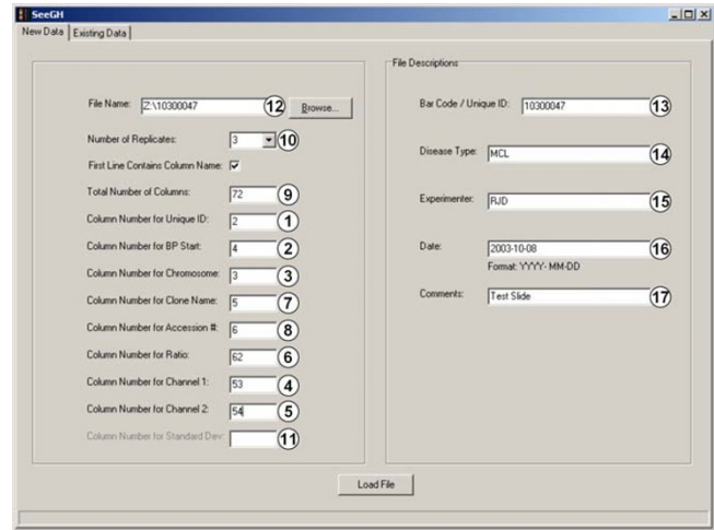
Figure 2 SeeGH "New Data" Window. Buttons correspond to descriptions in text.
