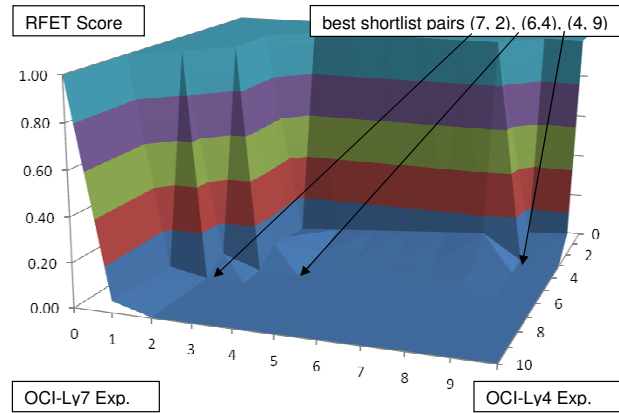
Figure 3 BLANKET applied to ranked list date of 190 descriptors from He et al. (He et al. 2005). BLANKET suggests that three combinations of shortlists are sufficiently coincidental to meet a p-value of .05. Note that each selected shortlist pair (p, q) has unequal numbers of descriptors selected from both experiments ( p \neq q ).
